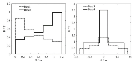
Figure 5: Magnetic field distribution of the dipoles.
