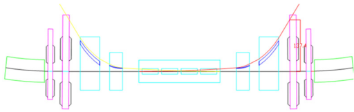
Figure 7: The injection and extraction system layout.
