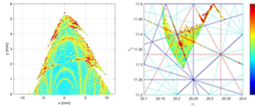
Figure 4: On-momentum FMA at the injection point.
