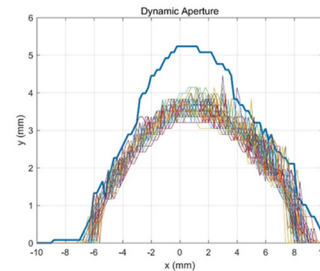
Figure 6: Dynamic aperture at injection point (100 seeds).
