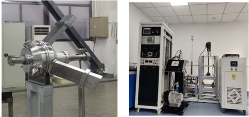
c) Aluminum cavity d) Vacuum coating facility
