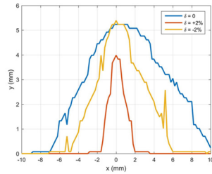
Figure 2: Dynamic aperture at the center of 1.5 GeV storage ring straight section.
