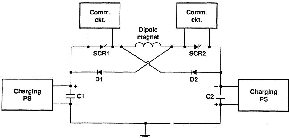
FIGURE 3 Forced Commutation Electrolytic Capacitor Bank and Silicon Controlled Rectifier-diode System.
