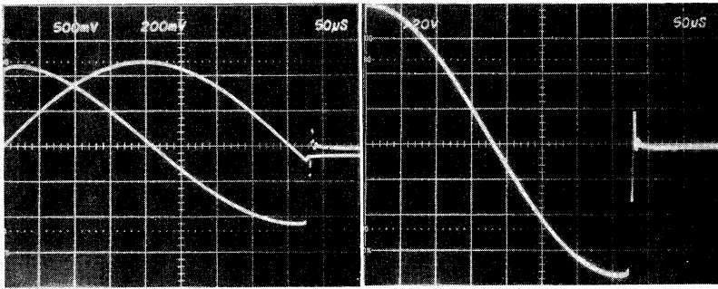
FIGURE 7 Current and Voltage Waveforms for H-type Dipole Magnet.
