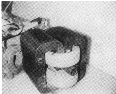
FIGURE 6 Pre-prototype 1/4-Scale H-type Dipole Magnet with SCR-Driven Bipolar Capacitor Bank.
