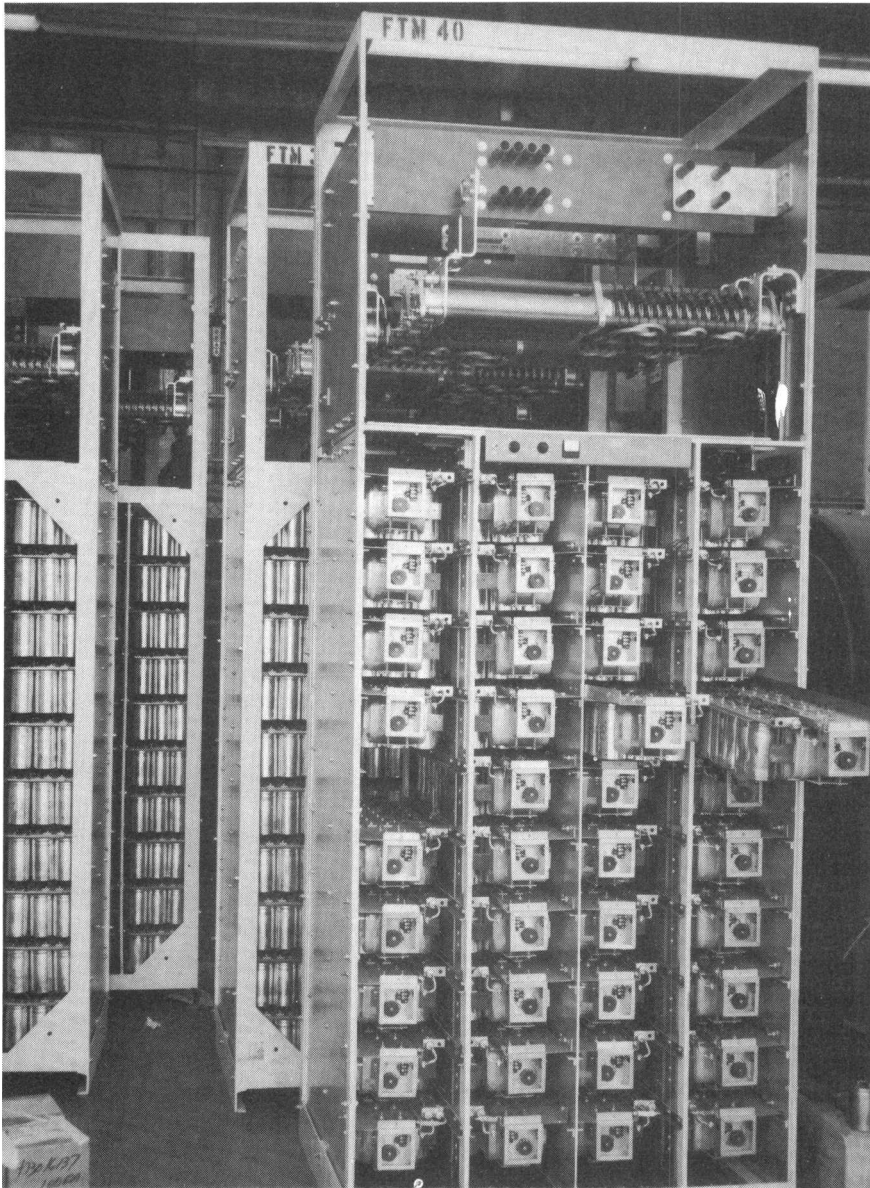
FIGURE 5 Six-MJ Electrolytic Capacitor Bank for Magnetic Fusion.
