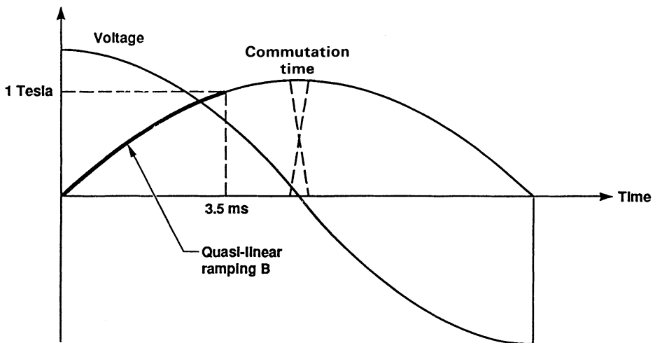
FIGURE 1 Voltage and Current Waveforms that Generate a Quasi-Linear Magnetic Field.
