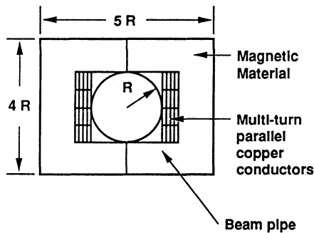
FIGURE 4 Approximate cross section of Dipole Magnet for Recirculating Heavy Ion Fusion Induction Accelerator.
