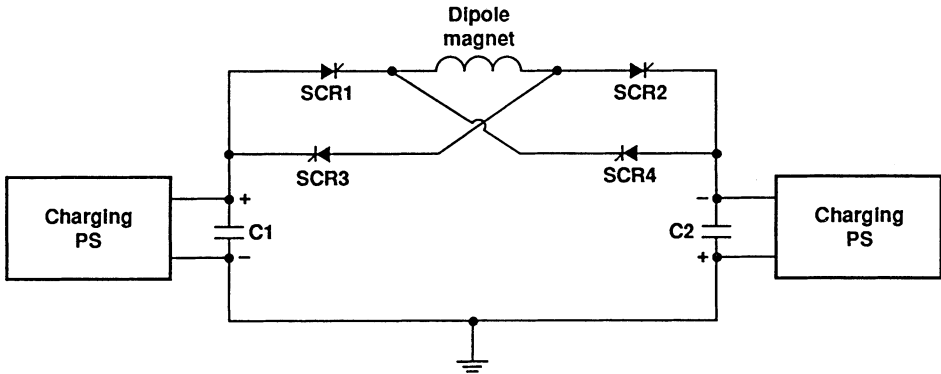
FIGURE 2 Self Commutating Bipolar Capacitor Bank and Silicon Controlled Rectifier System.
