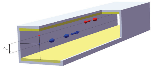
Figure 1: Conceptual design of a beam-driven short period FEL undulator.
