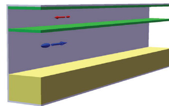
Figure 3: A rectangular waveguide beam driven undulator with a field concentrator. The high dielectric constant plate (green) separates the drive and undulator sections of the structure.
