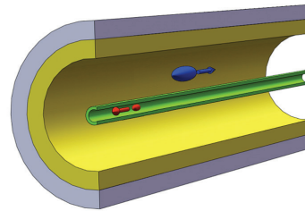
Figure 2: A beam driven undulator with a field concentrator. A cylindrical coaxial design with the undulating beam passing through the structure along the central axis.
