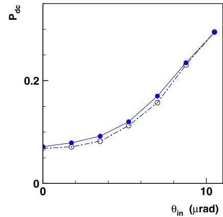
Fig. 4. (Color online.) The experimental dependence of the dechanneling probability of 400 GeV/c protons in the bent silicon crystal on the incident angle of the beam fraction \theta_{in} (filled circles). The simulation results are shown by the empty circles and dot-dashed line.
