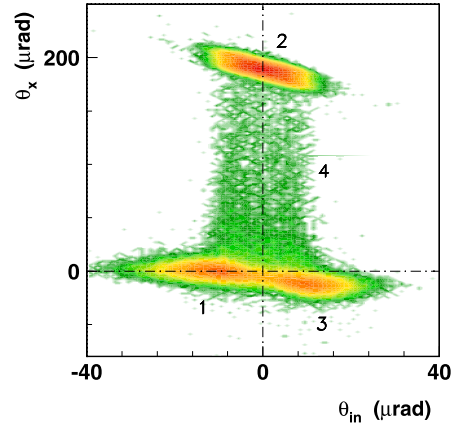
Fig. 2. (Color online.) The intensity distribution of 400 GeV/c protons passed through the bent silicon crystal when its orientation is optimal for channeling in the deflection angles \theta_x as a function of incidence angle \theta_{in} of particles relative to the (110) planes at the crystal entrance.
