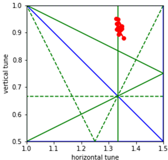
Figure 8: Tune diagram of PPR.
