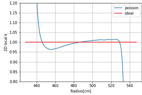
Figure 4: Two-dimensional local magnetic field gradient k_{local\_2D} as a function of radius.
