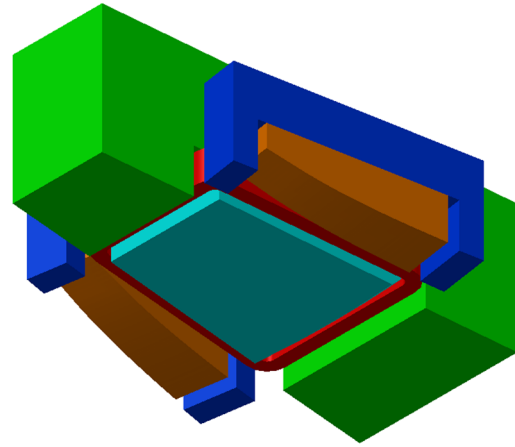
Figure 5: 3D model of the electromagnet of PPR.
