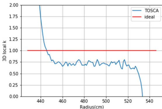
Figure 7: Three-dimensional local magnetic field gradient k_{local,3D} as a function of radius.
