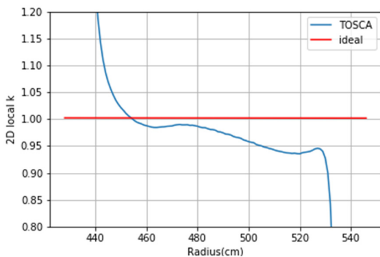
Figure 6: Two-dimensional local magnetic field gradient k_{local,2D} as a function of radius at the center of the F pole.
