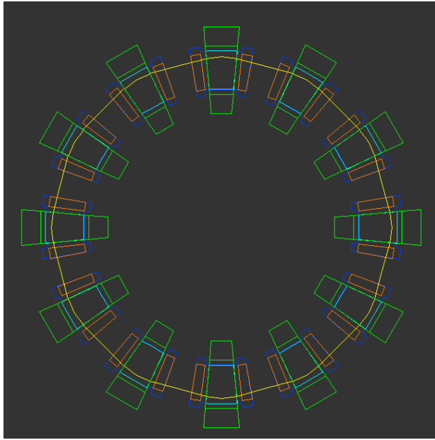
Figure 2: Arrangement of the electromagnets of PPR.
