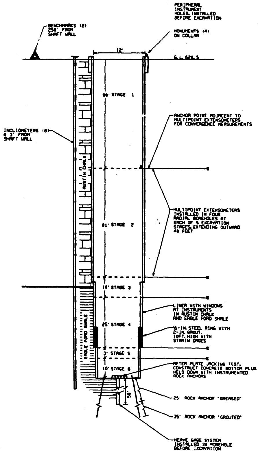
Figure 5 - Large Diameter Drilled Hole; Longitudinal Section
