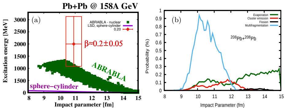
Fig. 2. (Colour on-line) (a) Excitation energy of the spectator in non-central ^{208}\text{Pb}+^{208}\text{Pb} collisions at 158 A GeV beam energy, computed in the abrasion-ablation model ABRABLA (green squares). The latter is compared to the excitation energy predicted by the geometrical model of sphere-cylinder collision (thick solid/purple line). The red rectangle gives the estimated kinetic energy range for the expanding charged sphere described in the text. The plot is redrawn from [13]. (b) Probability distribution in bins of impact parameter of the non-central ^{208}\text{Pb}+^{208}\text{Pb} reaction, obtained for our ABRABLA event sample and broken into different spectator de-excitation channels.
