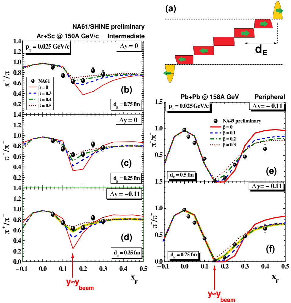
Fig. 1. (Colour on-line) (a) Schematic sketch of the ultrarelativistic nucleus–nucleus collision made according to the model [5]. (b), (c), (d) Ratio of the number of emitted \pi^+ over \pi^- measured in Ar+Sc collisions at intermediate centrality by the NA61/SHINE Collaboration [7]. The experimental data points are compared to model simulations described in the text. The different combinations of d_E , \beta and \Delta y are indicated in the plots. The combination which we judge to give the optimal description of the data is indicated by the thick light grey/yellow line. (e), (f) Similar comparison as for the three previous panels, made for peripheral Pb+Pb collisions measured by the NA49 experiment [8]. The optimal description of experimental data is indicated by the thick light grey/yellow line. The plots are redrawn from Refs. (a) [5], (b)–(d) [7], (f) [10].
