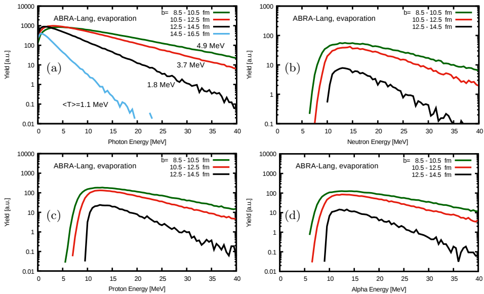
Fig. 3. (Colour on-line) Energy spectra of photons (a), neutrons (b), protons (c) and \alpha (d) in different ranges of impact parameter of Pb+Pb collisions at 158 A GeV beam energy. All the particles are emitted by the excited spectator produced in the collision by the ABRA part of the ABRABLA model, with the de-excitation process computed in the 4DLangevin approach. Average spectator temperatures, estimated from the excitation energies E^* using the formula T = (E^*/a)^{1/2} , are indicated in panel (a).
