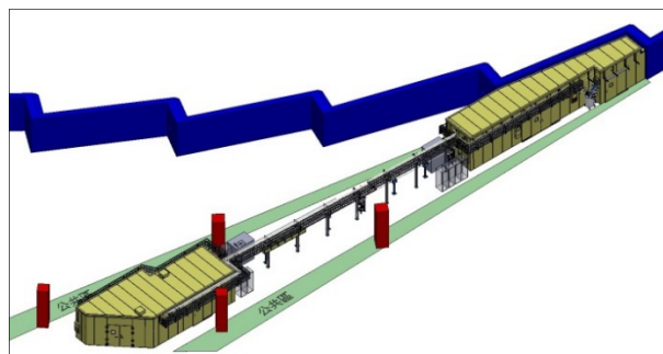
Figure 2: The picture of TPS Optics Hutch.
