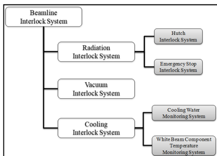
Figure 1: System architecture of Beamline Interlock System.
