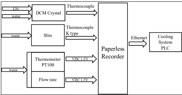
Figure 9: System architecture of Cooling System.
