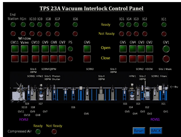
Figure 7: The picture of _Vacuum Interlock Control Panel.
