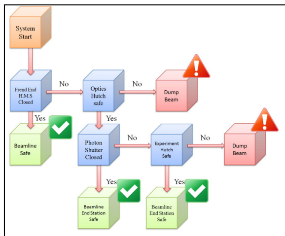
Figure 5: The picture of _active dump beam protection mechanism.
