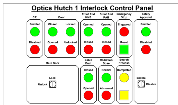
Figure 3: The picture of Optics Hutch Interlock Control Panel.
