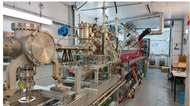
Figure 2: The injector test stand for MINERVA's front-end linac as it is today. The section in the middle with red pipes is the RFQ.
