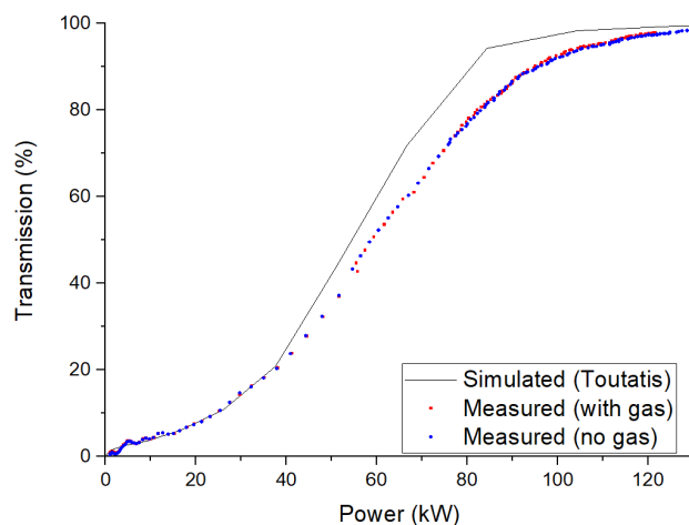
Figure 8: Measured RFQ transmission with and without Argon injection into the LEBT compared to simulations of a perfect model using the Toutatis software [14].
