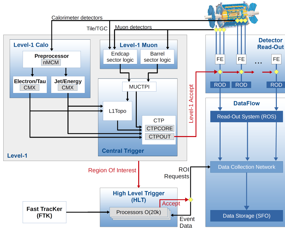
Figure 2.14: The ATLAS trigger system and data acquisition in Run 2.
