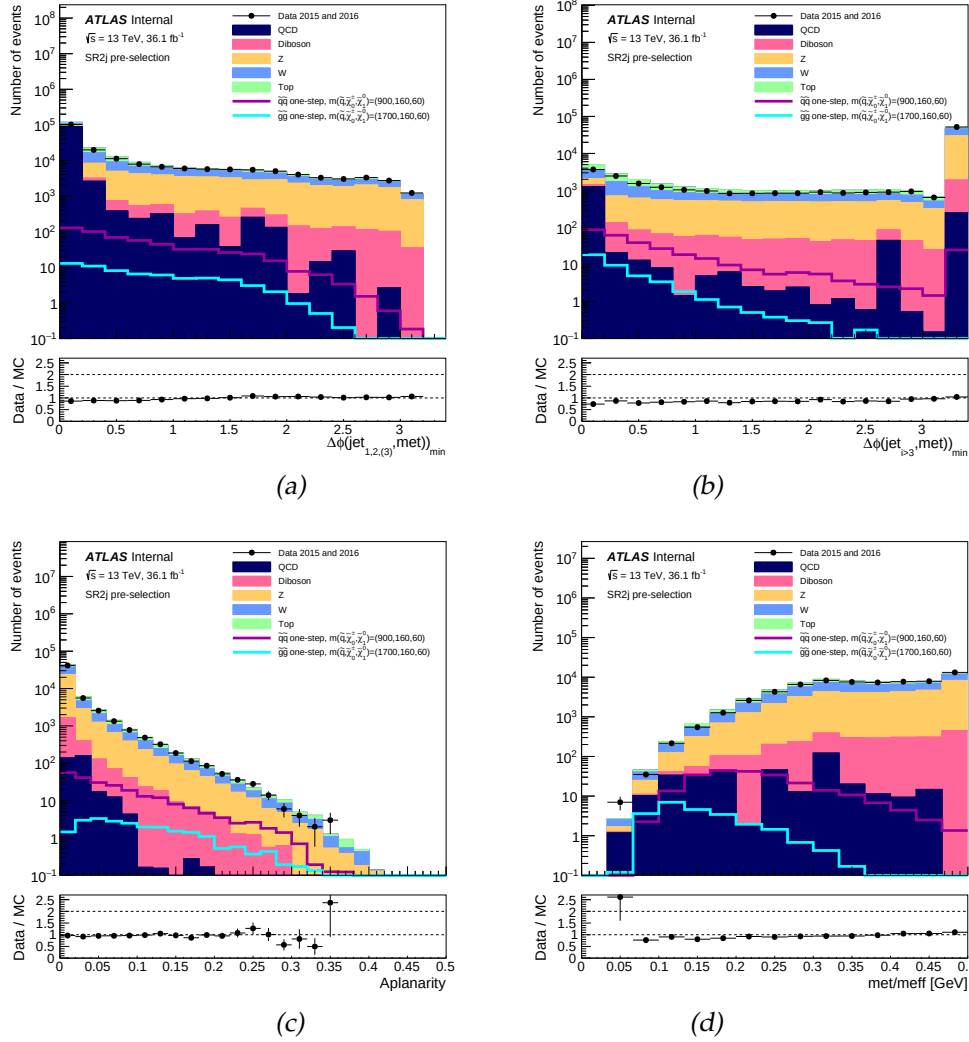
Figure 6.2: Distributions of \Delta\Phi (a), \Delta\Phi R (b), aplanarity (c), and \frac{E_T^{miss}}{m_{eff}^{Incl}} (d). A SR2j events pre-selection is applied except on \Delta\Phi on (a) and (b). No selections on \Delta\Phi are applied for (a), and the selection \Delta\phi(jet_{1,2,(3)}, E_T^{miss}) > 0.4 is applied on (b). Black points represent 2015 and 2016 data. The Monte Carlo background expectation normalized to 36.1 fb -1 is illustrated in coloured area. The purple and blue lines respectively show the distribution of \tilde{q}\tilde{q} and \tilde{g}\tilde{g} one-step signals decaying with intermediate chargino. The error bars show the statistical uncertainties.
