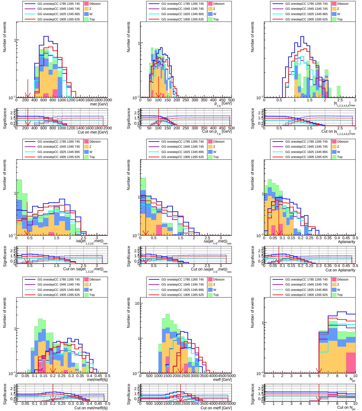
Figure 6.9: Distributions of discriminating variables in the signal region 6j-2200 using simulated events at \sqrt{s} = 13 \text{ TeV} . The Standard Model background expectation is illustrated in coloured areas and includes diboson, Z+jets, W+jets and top backgrounds. Various one-step decay signals with emission of two intermediate charginos (CC) are shown with coloured lines. At the bottom of the distributions, the signal significance as a function of the cut value is shown. The red arrows show the nominal selection of each variable in the signal region. Luminosity is normalised to 36.5 \text{ fb}^{-1} .
