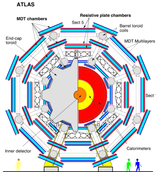
Figure 2.13: The ATLAS muon spectrometer.
