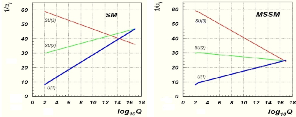
Figure 1.4: Evolution of the coupling constant as a function of the energy scale (log scale). On the left, the coupling constants of the Standard Model do not converge. On the right, coupling constants of the Minimal Supersymmetric Standard Model can be unified at the Grand Unification scale [25].
