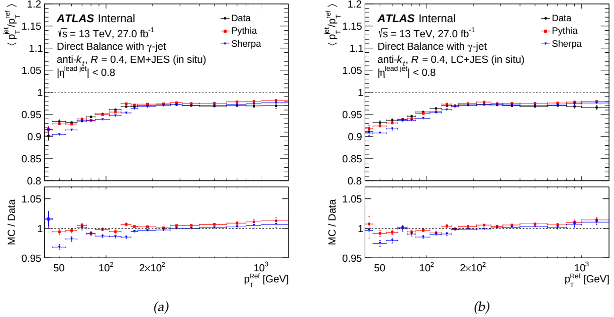
Figure 4.26: Ratio \langle p_T^{jet} / p_T^{ref} \rangle for jets fully calibrated at EM+JES scheme (a) and LC+JES scheme (b), with 2015 data using the \gamma +jet Direct Balance technique, as a function of p_T^{ref} for both data and MC simulation. Jets are selected in the central region of the hadronic calorimeter |\eta^{leadjet}| < 0.8 . Error bars indicate the statistical uncertainties.
