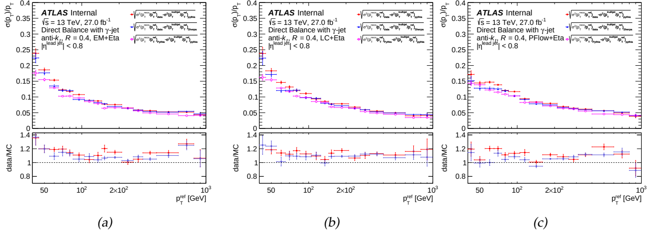
Figure 5.4: Jet energy resolution as a function of p_T^{\text{ref}} with EM (a), LC (b) and EMPFlow (c) jets calibrated up to the \eta -intercalibration, using 2016 data and Pythia8 (red points), 2016 data and Sherpa2.2 (up triangles), and Pythia8 only (pink circles). The width of the distributions are estimated with a Gaussian fit. The bottom graph shows the ratio between the JER extracted from data and MC, and the JER extracted from MC only, for both Pythia8 and Sherpa2.2. Error bars show the statistical uncertainties of the fit.
