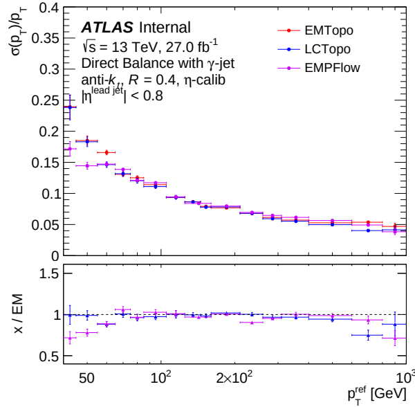
Figure 5.5: Comparison of the jet energy resolution between EM (a), LC (b) and EMPFlow (c) jets calibrated up to the \eta -intercalibration as a function of p_T^{\text{ref}} using 2016 data. The bottom graphs show the ratio between resolution of LC and EM jets (blue), and between EMPFlow and EM jets (pink). Error bars show the statistical uncertainties.
