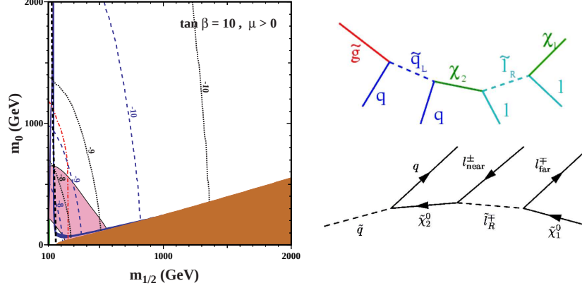
Fig. 1. The bottom triangular area is theoretically excluded (the LSP is the lightest stau and is thus charged); the light (bottom-left) area is favored by g-2 ; the dark line area is favored by WMAP. The spin-independent elastic-scattering cross-sections are also shown and labeled by their exponents in units of picobarns. Generic decay chains originating from a gluino (right, top) or a squark (right, bottom).
