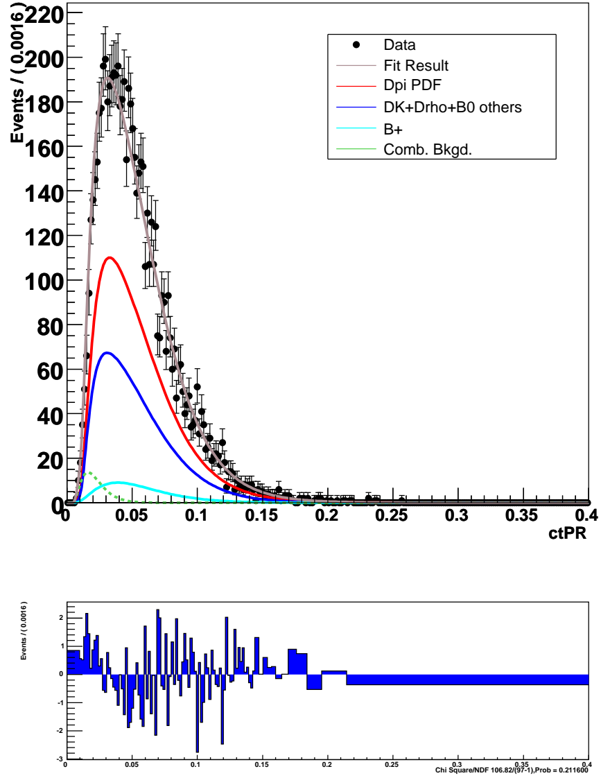
Figure 9.8: ct projection of the lifetime fit to events reconstructed as B^0 \rightarrow D^{*-} \pi^+ in the combined FR+PR region.
