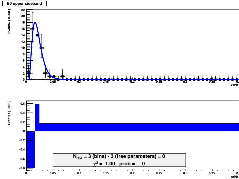
Figure 9.7: Background model for B^0 \rightarrow D^{*-}\pi^+ from the upper sideband data with m_B \in [5.7, 6.4] GeV/ c^2 .
