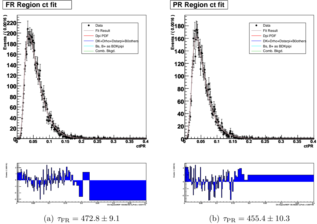
Figure B.3: Results for the fits to the FR(left) and PR(right) regions of the B^0 \rightarrow D^-(K^+\pi^-\pi^-\pi^+) sample with the default cuts + \pi_B trigger requirement + L_{xy}(B \rightarrow D) > 500 \mu\text{m}
