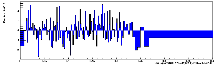
Figure 9.20: ct projection of the lifetime fit to events reconstructed as B^+ \rightarrow \overline{D}^0 \pi^+ in the combined FR+PR region.
