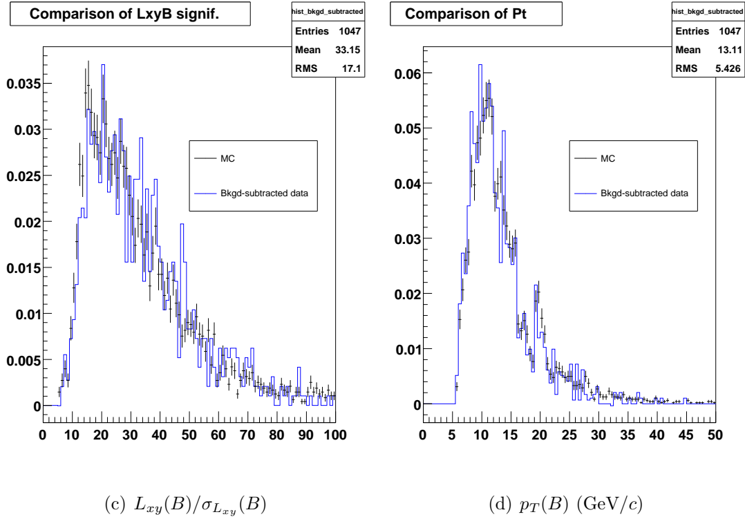
Figure 7.10: Comparison between B_s \rightarrow D_s^- (\phi \pi^-) \pi^+ simulation and data
