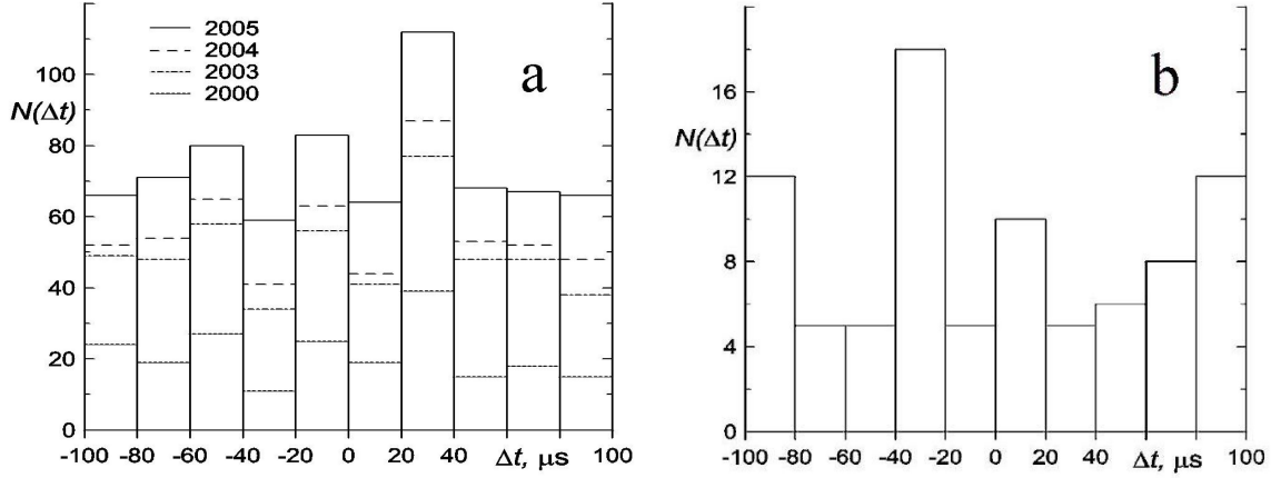
Fig. 1. Distributions N(\Delta t) of pair events on their time shift relative to the upper screen HPSs. (a) The sum of Marches 2000, 2003, 2004, and 2005. The +30\mu s maximum exceeds the mean level by 33 events; its significance is 3.63\sigma (C.L. > 99.97\% ) [14]. (b) The underground Baksan experiment [15]. The photo-cathode of the bottom PMT, which is sensitive to daemon passages due to its thick 1\mu m inner Al coating, is screened with Al foil. Observations during September 3-11, 2005; 86 events altogether. Significance of the -30\mu s maximum is 2.2\sigma .
