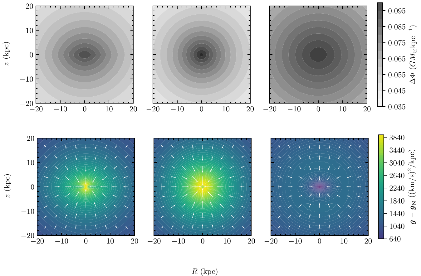
Figure 9. Top row: Gravitational potential difference between the Newtonian baryon-only model and other models ( \Delta\Phi = \Phi_N - \Phi_{\text{model}} ). The left-hand, middle, and right-hand panels are for the QUMOND, DM, and MOG cases, respectively. Generally the MOG model is not favoured by our Jeans-equations tests. At present, it is yet an open question to what degrees DM and MOND, respectively, represent the real gravitational field of the MW. Bottom row: The corresponding field-strength difference between the Newtonian baryon-only model and other models, \mathbf{g}_{\text{model}} - \mathbf{g}_N . The direction of the vectors is denoted by arrows, and their magnitude is colour coded. Note that around the centre, the darker the MOG’s extra gravity is (in blue and even purple) the weaker is the field strength.
