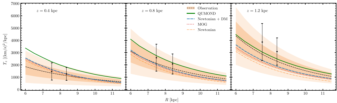
Figure A3. As Fig. A2, but showing the T_z test results.
