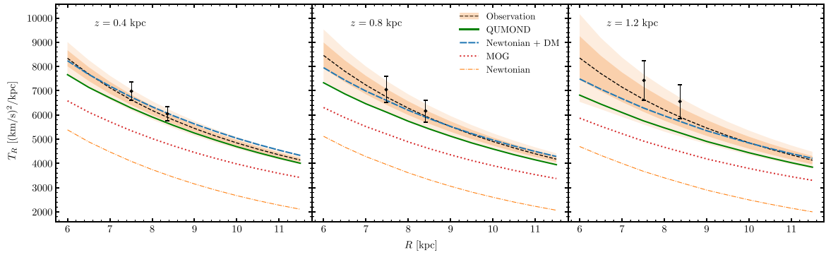
Figure A2. As Fig. 2, but showing the T_R test results for the ‘Weaker R_0 prior’ mass model of McMillan (2017). Also plotted is the results based on the RAVE sample (black dots with \pm 1\sigma error bars).
