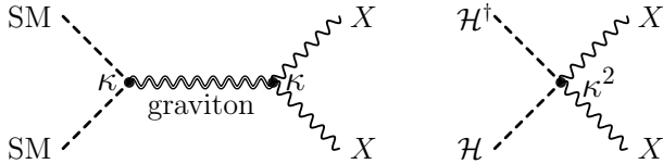
Fig. 1. Feynman diagrams that arise from (4). The left panel shows annihilation process for SM particles to vector DM X_\mu via the s -channel graviton exchange while the right panel shows contact interaction induced by the dim-6 operator.
