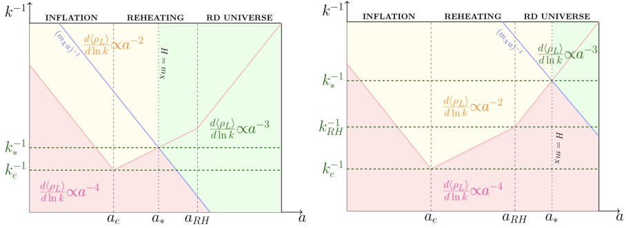
Fig. 3. Scaling of the energy density as a function of the scale factor for heavy i.e. H_{\text{RH}} < m_X (left diagram) and light H_{\text{RH}} > m_X (right diagram) vector DM. The main contribution to the total energy density comes from the mode k_* \equiv a(\tau : H = m_X)m_X . Here, k_e \equiv a_e H_e and k_{\text{RH}} \equiv a_{\text{RH}} H_{\text{RH}} .
