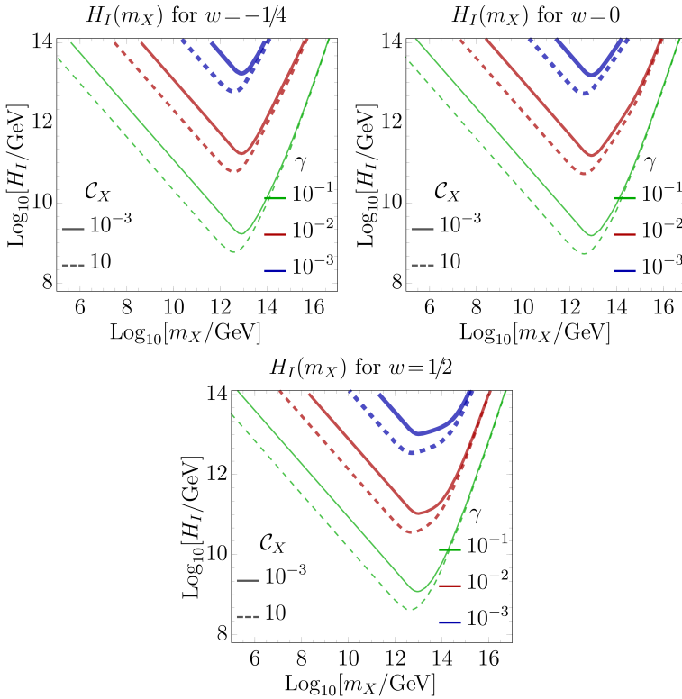
Fig. 2. Relations between the Hubble rate at the end of inflation H_I and vector DM mass m_X that reproduces the observed relic abundance \Omega_{\text{DM}}^{\text{obs}} h^2 .
