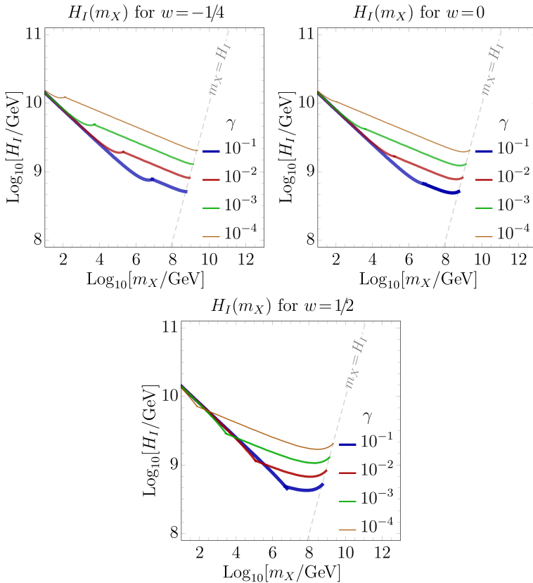
Fig. 4. Relations between the Hubble rate at the end of inflation H_I and vector DM mass m_X that reproduces the observed relic abundance \Omega_{\text{DM}}^{\text{obs}} h^2 .
