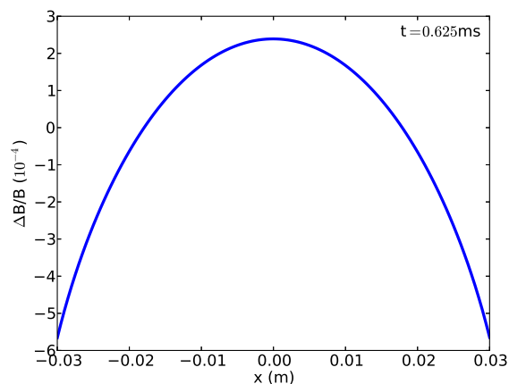
Figure 6: Field quality on the centre plane at peak field ( B=1.5\text{T} ).
