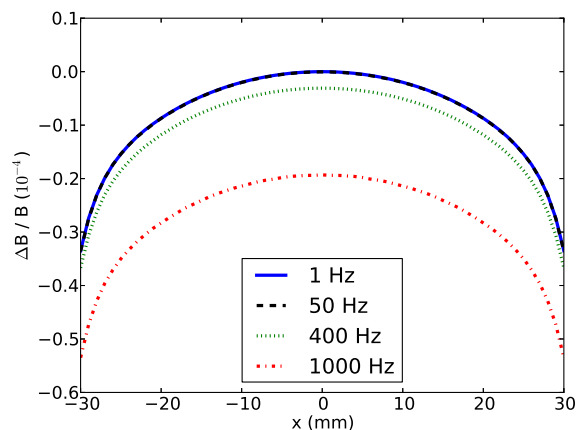
Figure 8: Field uniformity in the mid plane due to the eddy current losses as function of the frequency.
