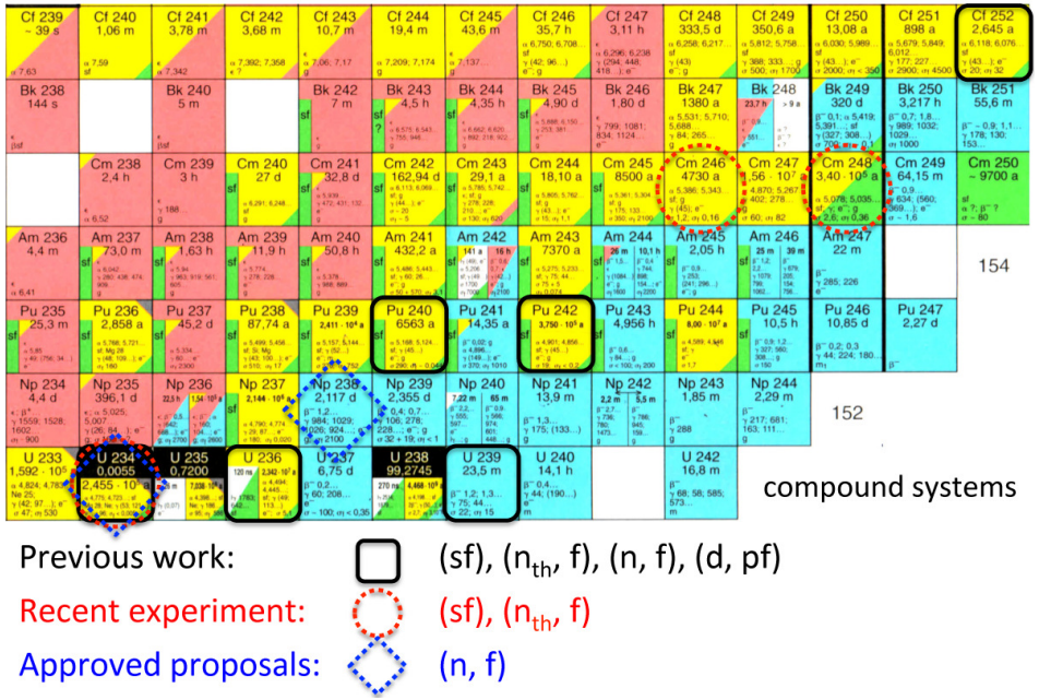
Fig. 1. Overview of compound systems, whose fission process was investigated by us during the past years as well as ongoing and planned work. Here, it is also indicated, whether it was spontaneous or induced fission, and in the case of the latter which reaction was employed.
