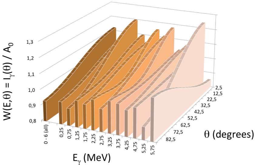
Fig. 2. Pseudo-3D plot of the fit results to the measured angular distributions of prompt \gamma rays from ^{252}\text{Cf}(\text{sf}) according to Eq. (1). Shown is the angular distribution obtained for the entire energy spectrum to the left together with those for the individual energy bins. Please, observe that for the latter, the axis description gives the center of each bin.
