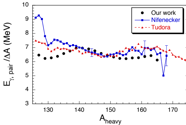
Fig. 3. Total \gamma -ray energy for a pair of fission fragments as a function of the heavy fragments mass. Our preliminary experimental results, denoted as black dots, were obtained for mass bins \Delta A > 1 due to the limited mass resolution of the FGIC (see the text for details). They are compared to data from Ref. [26] and values calculated with the Point-by-Point model [27], represented by squares and triangles, respectively.
