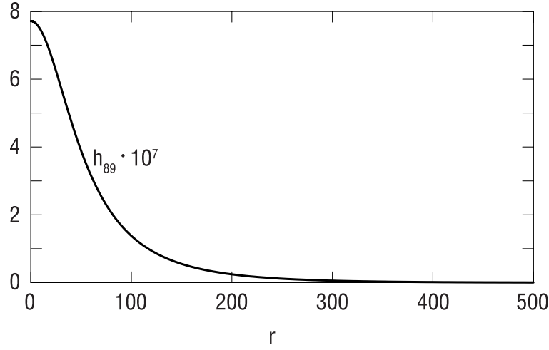
Figure 9. Core-mode field of the scalar metron solution.
