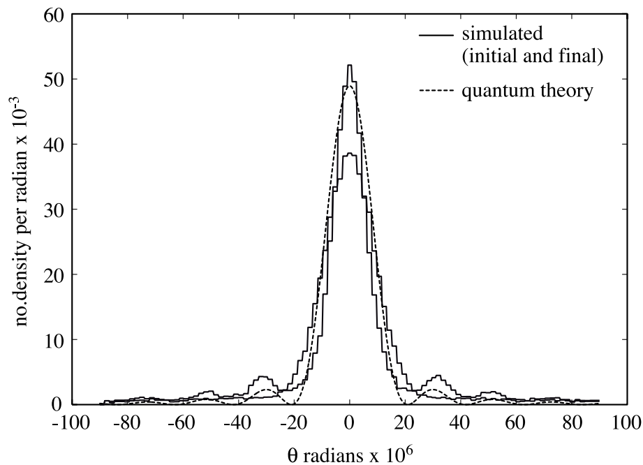
Figure 14. Quantum theoretical and metron particle distributions for a monochromatic particle beam diffracted at a single slit.
