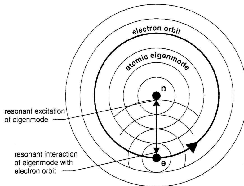
Figure 15. Metron model of electron orbiting an atomic nucleus. The low-frequency field produced by the difference interaction between the primary core-mode field of the electron and the secondary core-mode field scattered at the atomic nucleus modifies the electron orbit. Resonance between the electron orbit and the difference-frequency field produces trapping of the electron in discrete orbits in accordance with Bohr's original discrete-orbit model. The resonant scattered core-mode fields correspond to the QED eigenmodes (reproduced from [27]).
