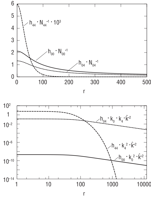
Figure 10. Wave-guide fields of the scalar metron solution. Top panel: linear fields; bottom panel: log-log plot ( k \equiv \kappa ; N_{44}, N_{00} are normalization factors).
