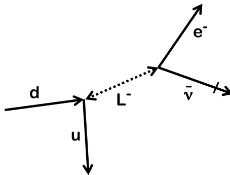
Figure 11. Metron picture of weak interactions resulting from the coupling of a left-spinor background wave field L^- with left-spinor core-mode components, illustrated for neutron decay. Cross-bars denote complex conjugate fields (in the limit of zero mass, this is identical to the anti-particle).
