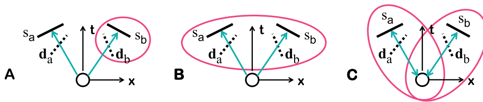
Figure 1. Alternative interpretations of the EPR experiment. A: a hidden-variable local model (disentangled, in disagreement with experiment); B: the quantum theoretical picture of space-like entanglement; C: a time-symmetrical classical model with past-future entanglement.
