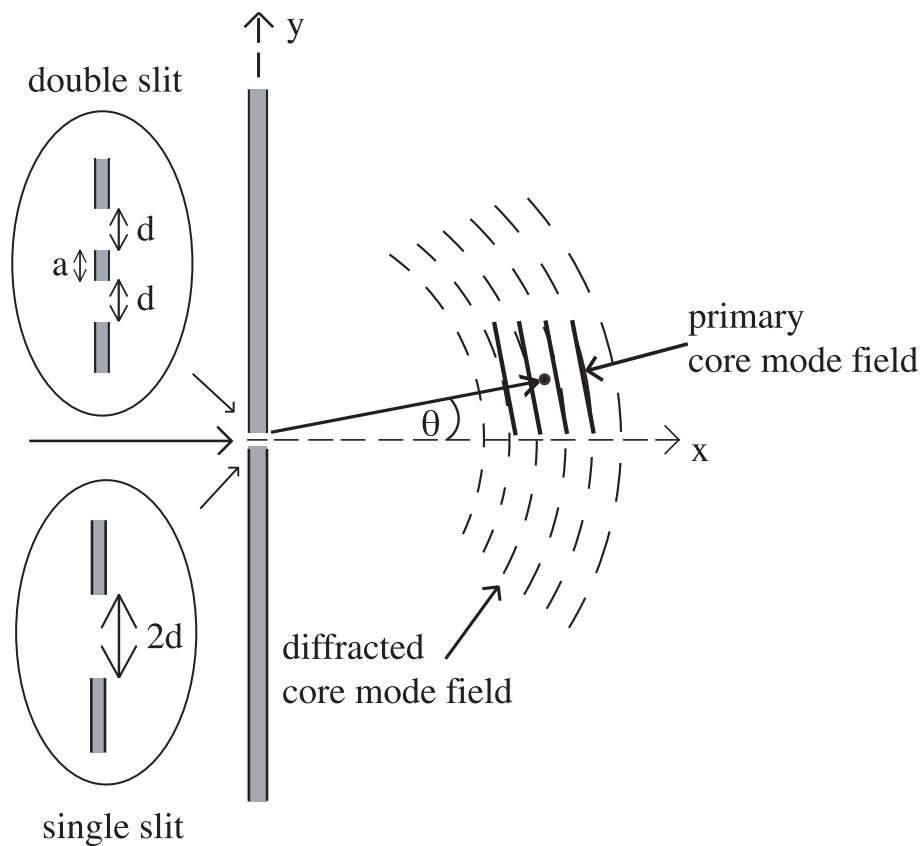
Figure 12. Interacting primary and diffracted fields of the metron model.
