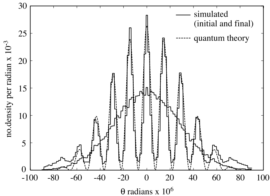
Figure 13. Quantum theoretical and metron particle distributions for a monochromatic particle beam diffracted at a double slit.
