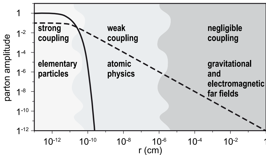
Figure 4. Near- and far-field components of metron solutions. Full line: core modes (fermions), decreasing exponentially for large r ; dashed line: wave-guide fields (massless bosons), decreasing asymptotically as 1/r .
