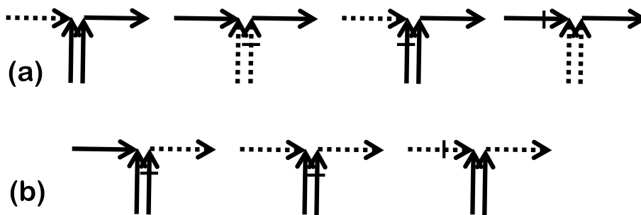
Figure 8. Interactions ensuring stability and uniqueness of the soliton solutions.
