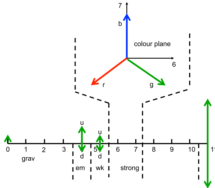
Figure 5. Wavenumber components ( k_0, k_4 - k_7, k_{11} ) of fermions (leptons and up and down quarks). Each fermion is composed of mirrored core-mode pairs with equal wavenumber components k_L for L < 11 and opposite wavenumber components \pm k_{11} .
