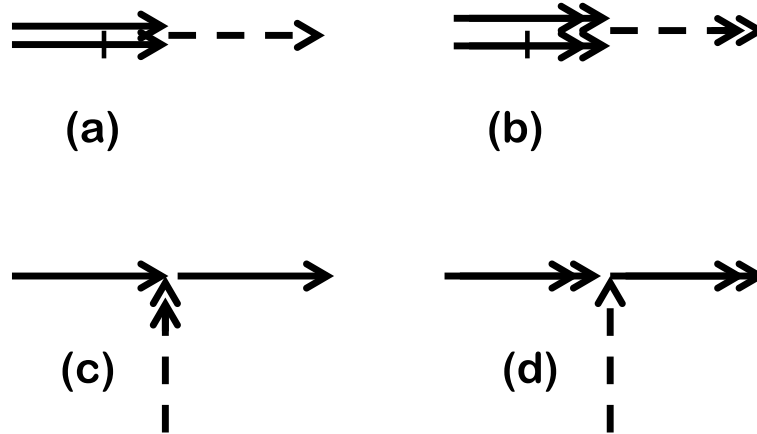
Figure 6. Panels (a), (b): generation of wave-guide fields (dashed arrows) by quadratic interactions of core modes (full arrows) and mirrored core modes (double-headed arrows). Cross-bars denote complex-conjugate fields (not anti-particles). Panels (c), (d): feedback of wave-guide fields on the eigenvalues of core modes. The dominant feedbacks are cross-interactions between core modes and wave-guide fields generated by mirrored core modes.
