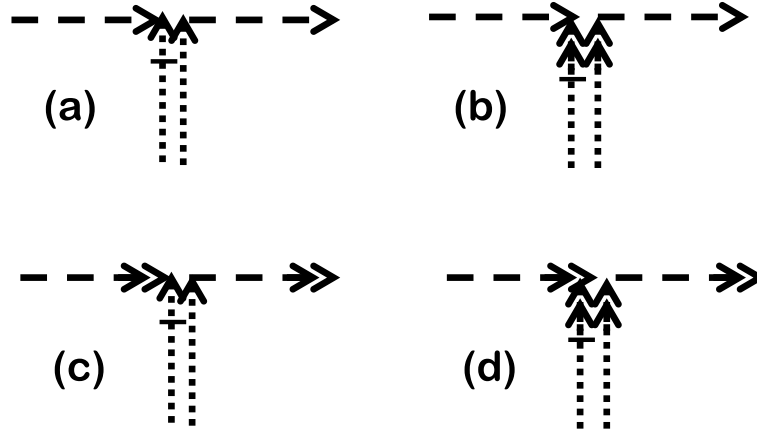
Figure 7. Selective damping of KSS fields (dashed arrows) through interactions with background wave fields (dotted arrows). Panels (a), (b): damping of KSS fields by cubic interactions with the background wave fields and their mirrored partners. Panels (c), (d): analogous diagrams for the damping of the mirrored KSS fields.
