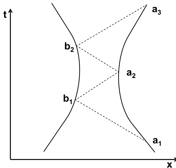
Figure 2. Past-future entanglement in relativistic time-symmetrical systems. The acceleration of particle a at position a_2 depends on the states of particle b at both positions b_1 and b_2 on the backward and forward light cones (dashed lines), respectively. The interactions a_1 \leftrightarrow b_1, b_1 \leftrightarrow a_2, a_2 \leftrightarrow b_2, b_2 \leftrightarrow a_3 represent a local time-symmetrical transfer of four-momentum in accordance with the relativistic generalization of Newton's third law actio = reactio .
