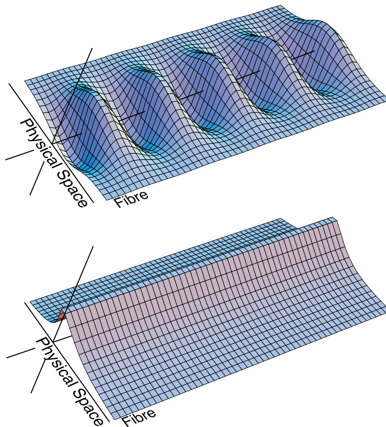
Figure 3. Schematic diagram of the periodic trapped-mode (upper panel) and wave-guide (lower panel) components of a metric soliton in the product space \text{physical-space} \times \text{fibre} (from H ). The trapped core modes are periodic also with respect to time.
