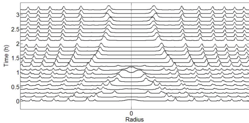
Figure 5: A family of intensity plots expressing the fringe pattern and its variation in time
