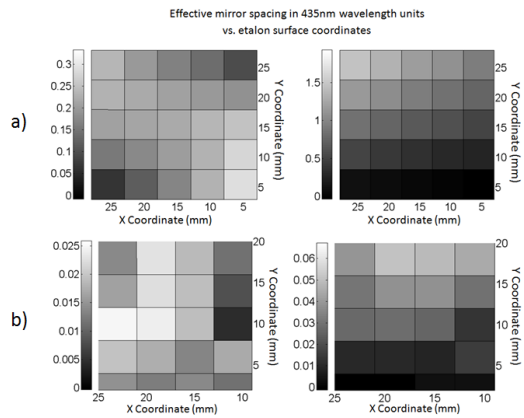
Figure 7: a) Prototype 13 mm etalon b) Commercial 5 mm etalon. Left: Map of the effective etalon spacing (in units of 435 nm wavelength) with deviation from parallelism removed to reveal the etalons flatness. Right: Map of the effective etalon spacing.
