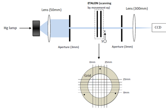
Figure 6: Experimental setup for the characterization of the Fabry-Perot etalon with respect to its Flatness.
