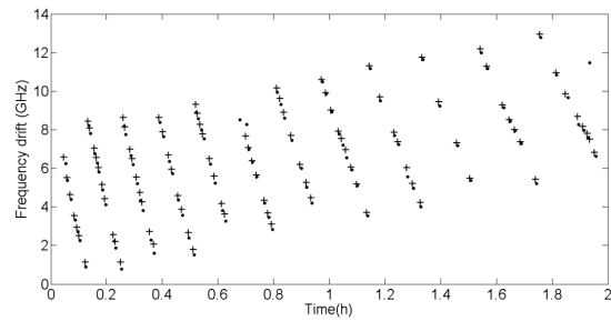
Figure 3: Plot of the frequency drift vs the elapsed time from the moment the laser started to operate.
