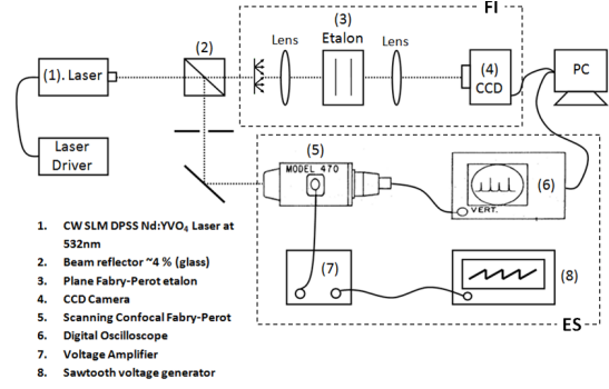
Figure 2: The experimental setup for the characterisation of the Nd:YVO 4 Laser.
