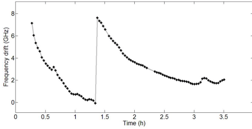
Figure 4: Plot of the relative Frequency of the most intensive laser mode vs. the elapsed time from the moment the laser started to operate.
