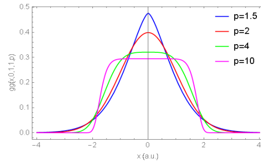
Figure 1: Comparison of ggGaussian distribution with different p value when the other parameters are the same.
