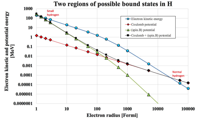
Fig. 2. Comparison of electron kinetic energy T_{\text{kinetic}} , and absolute values of V_{\text{Coulomb}} , V_{(\text{Spin.B})} and (V_{\text{Coulomb}} + V_{(\text{Spin.B})}) potentials.
