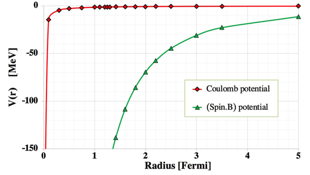
Fig. 1. V_{\text{Coulomb}} and V_{(\text{Spin.B})} potential shapes as a function of radius close to proton.
