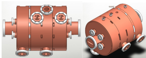
Figure 3: TM020 4-cell harmonic cavity for EBS [11].
