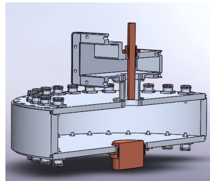
Figure 4: ESRF 1.41 GHz TM030 cavity combiner.
