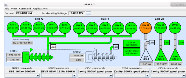
Figure 2: Graphical control synopsis of the EBS RF system, here in a fall back configuration with only 12 cavities in operation at 200 mA.
