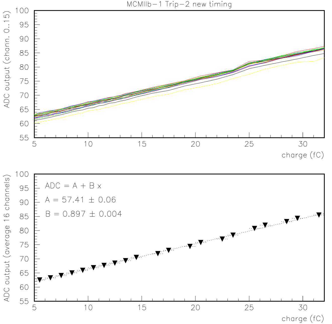
Figure 13: Calibration of ADC readout. The upper plot shows the analog readout for different values of the injected charge, for 16 channels in MCMIIb-1-Trip2. The lower plot shows the average of the 16 channels, together with a linear fit giving the calibration constant B = (0.897 \pm 0.004) counts/fC.
