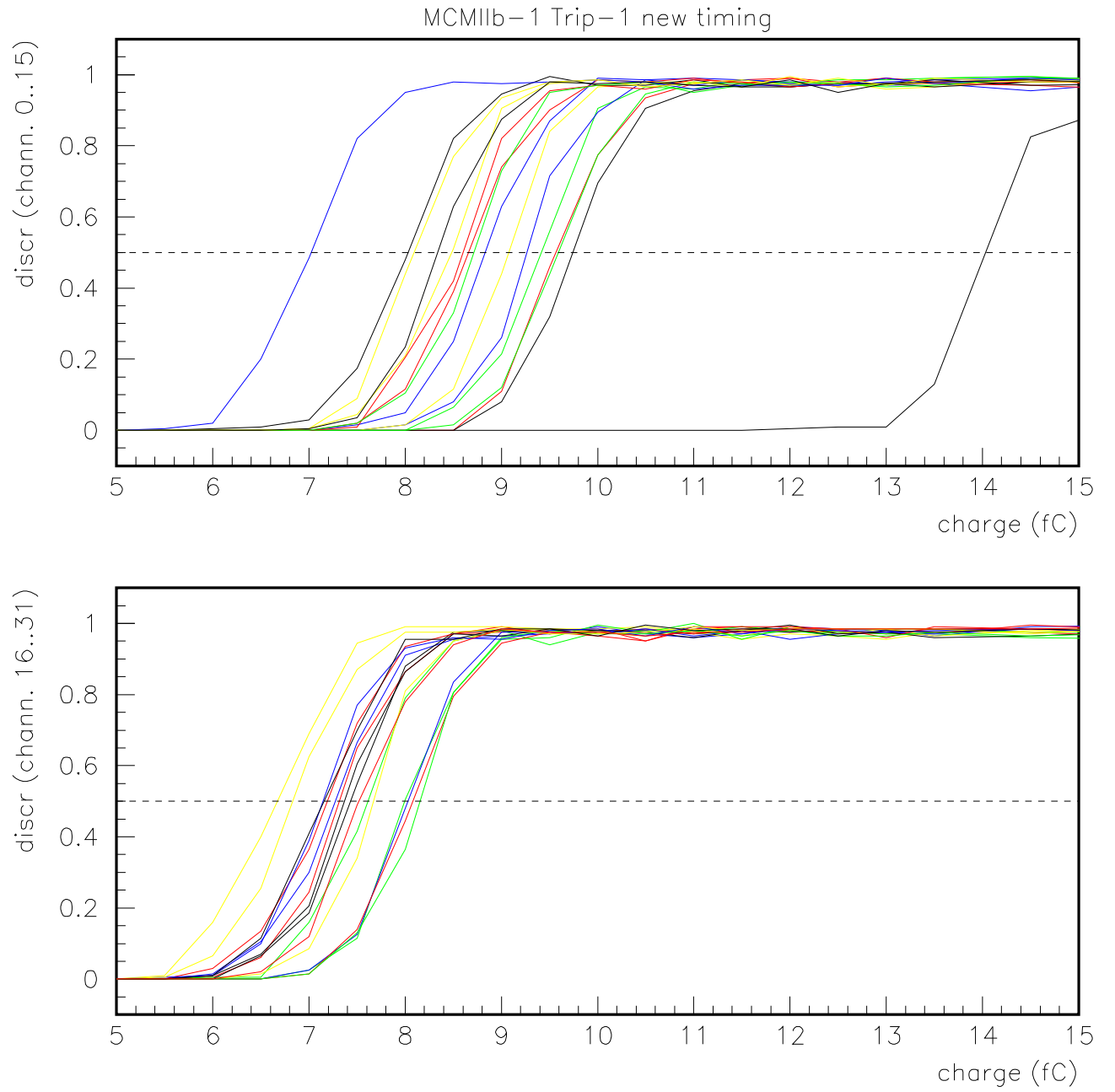
Figure 14: Discriminator scan for MCM1-trip1, for Option (B)
