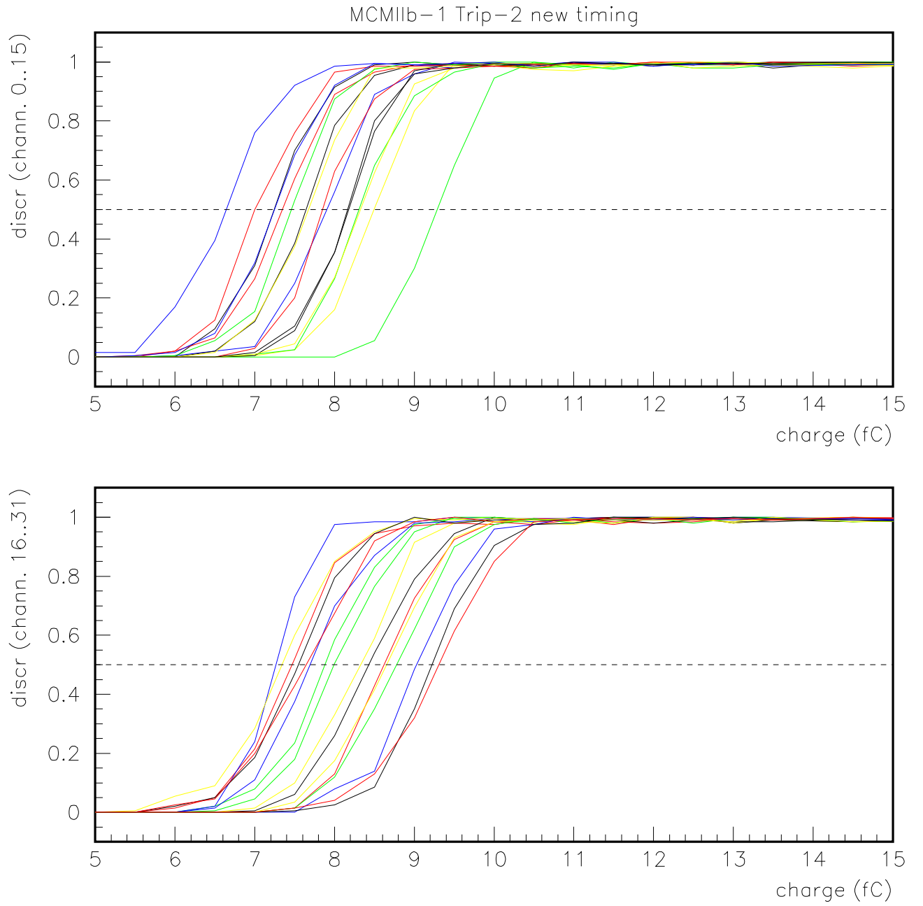
Figure 15: Discriminator scan for MCM1-trip2, for Option (B)
