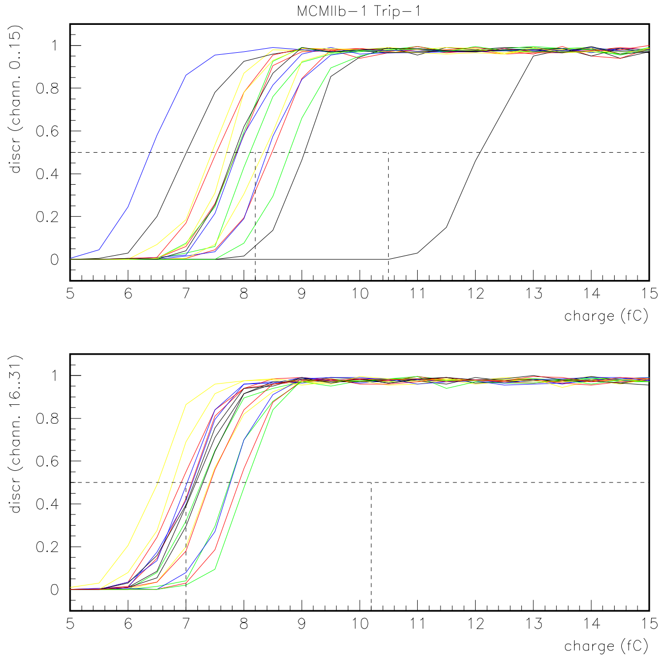
Figure 1: Discriminartor scan for MCMIIb-1-Trip1.
