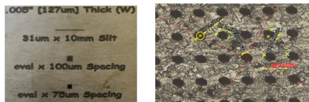
Figure 3: Laser drilled arrays of holes in tungsten.
