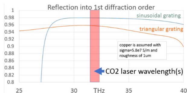
Figure 5: Comparison of grating efficiency (simulation).
