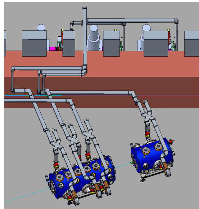
Figure 5: The gun module is on the right and the booster module on the left. Behind the radiation shield wall the klystrons can be seen.
