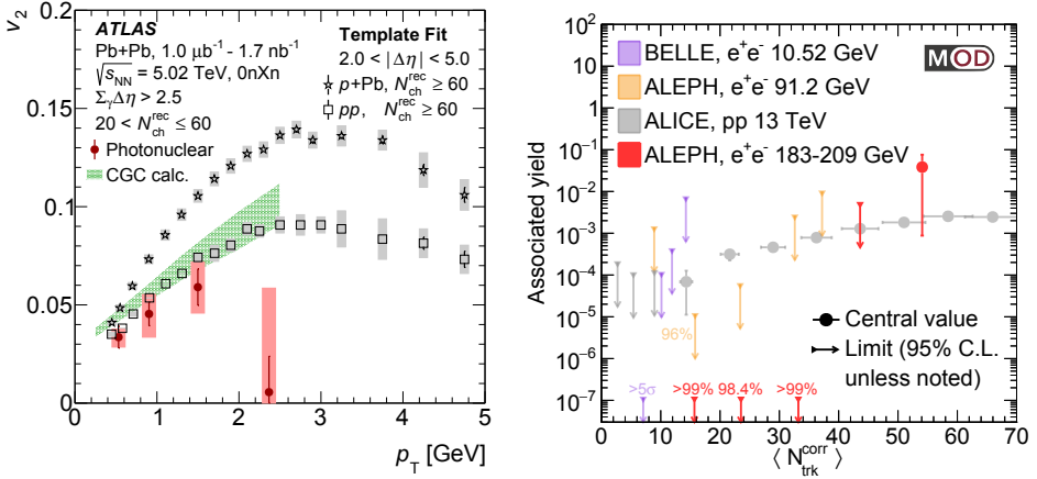
Figure 1. On the left: v_2 for charged particles in \gamma -Pb (red), pp (black squares), and p-Pb (black stars) collisions measured by the ATLAS Collaboration. The color glass condensate expectation are shown with a green band. Figure from [2]. On the right: charged particles yields associated to the near side peak of two-particle correlations in electron-positron [4] (coloured points) and pp [3] (grey) collisions.
