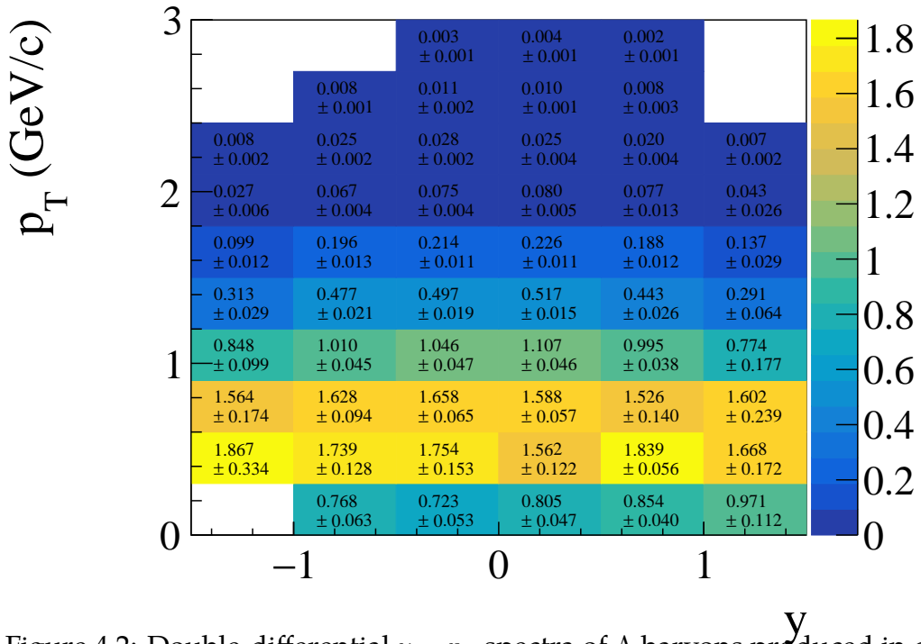
Figure 4.2: Double-differential y - p_T spectra of \Lambda baryons produced in central Ar+Sc collisions at 75A GeV/c beam momentum with statistical ( top ) and systematic ( bottom ) uncertainties provided in the form: (d^2n/dydp_T \pm \sigma_{stat}) or (d^2n/dydp_T \pm \sigma_{syst}) , respectively.
