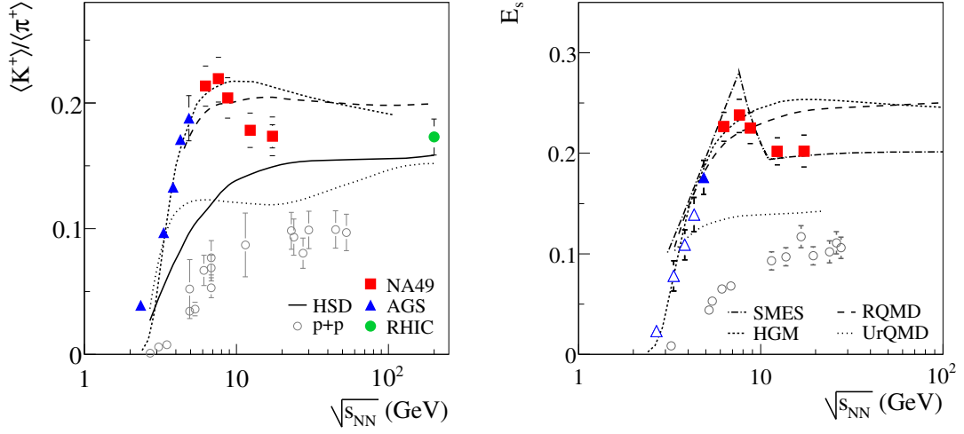
Figure 1.7: Energy dependence of \langle K^+ \rangle / \langle \pi^+ \rangle ratio ( left ) and strangeness enhancement E_s ( right , as defined by Eq. 1.3) observed by the NA49 experiment in Pb+Pb collisions (figures taken from Ref. [43]). Both quantities exhibit a sharp maximum at SPS energies, followed by a plateau towards RHIC energies, unlike p+p collisions, which show no peak. This behaviour is suggested to be compatible with transition to QGP.
