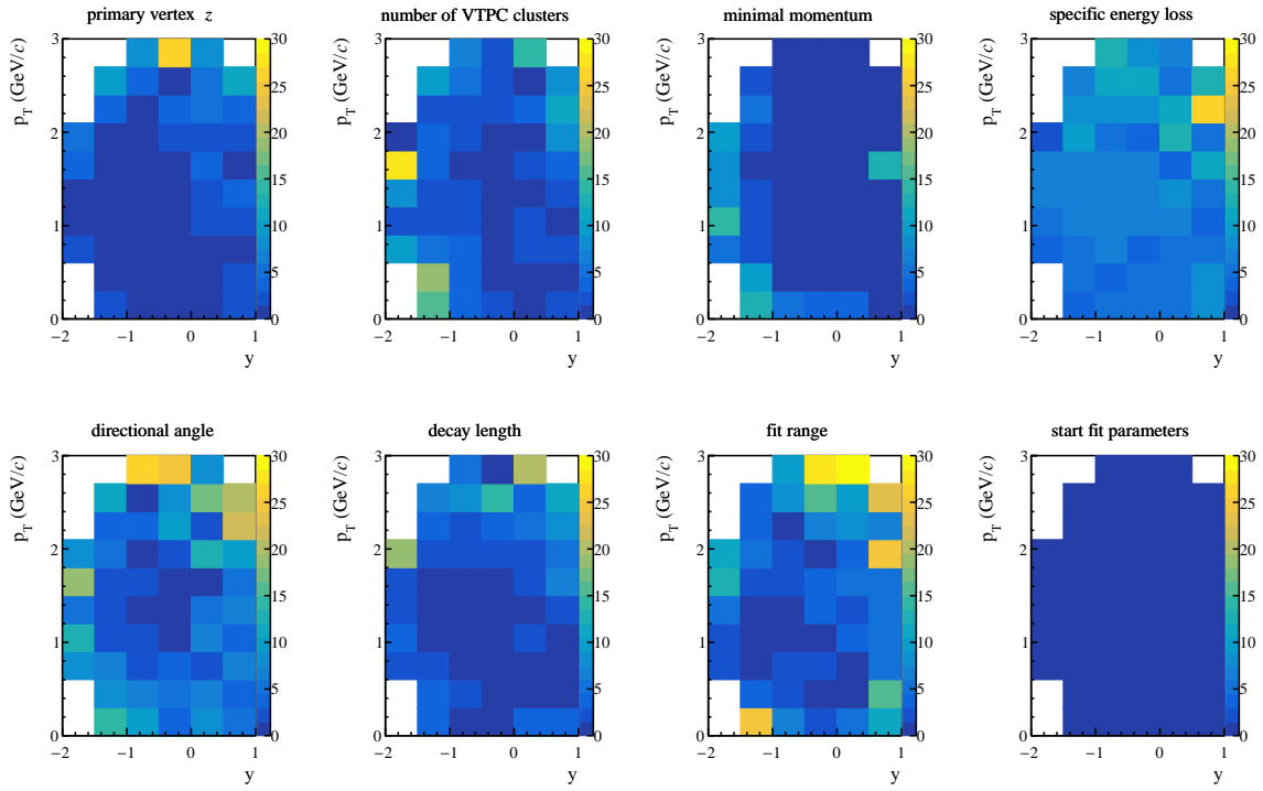
Figure 3.17: 150A GeV/c
