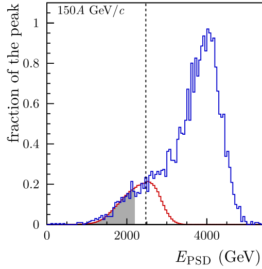
Figure 3.5: Energy E_{PSD} distribution as measured by the PSD calorimeter for 150A GeV/c beam momentum. The blue histogram represents minimum-bias selected events, while the red histogram corresponds to central trigger selected events, with histograms being normalized to align in the overlap region (left of the dotted line). The shaded area indicates the 10% of collisions with the lowest E_{PSD} values [73], which are accepted for the analysis.
