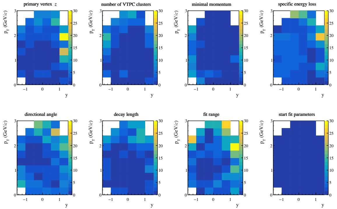
Figure 3.16: Contributions of selection criteria to the final systematic uncertainty of double-differential y - p_T spectra of \Lambda baryons produced in central Ar+Sc collisions at 75A GeV/c beam momentum.
