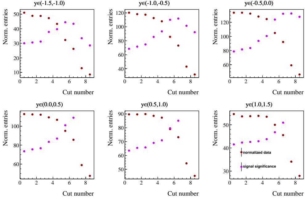
Figure 3.13: Example distributions of signal significance (magenta points) and signal yield (brown points) as a function of directional angle selection values in Ar+Sc collisions at 75A GeV/c after event and track selection. The signal yield distribution is scaled to match the integral of the signal significance distribution. The tested values for the criterion during the selection optimization are provided in Table 3.5.
