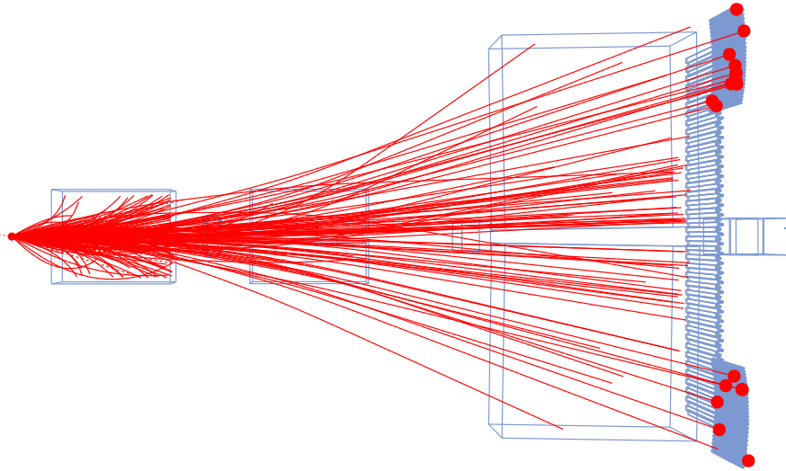
Figure 3.2: Visualization of reconstructed Ar+Sc collision at 75A GeV/c. The red lines depict reconstructed tracks along with red points as hits in TOF.
