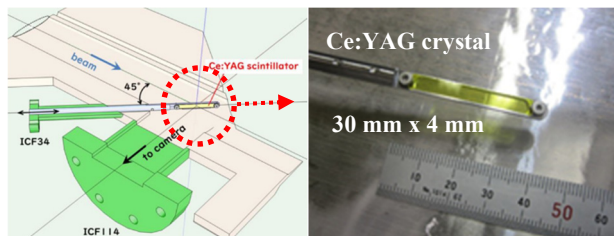
Figure 4: Newly developed small beam profile monitor using ICF34 port.
