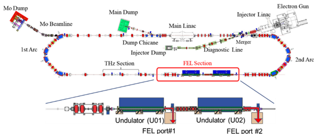
Figure 1: Layout of the cERL after modification for IR-FEL (upper) and enlarged drawing of the undulators installed in the south-straight section (lower).
