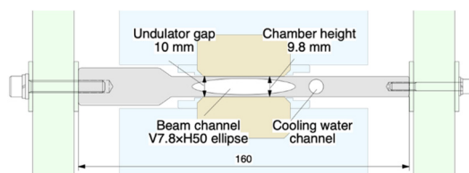
Figure 3: Cross section of the undulator beam duct. The undulator duct is made of extruded aluminum pipe with an opening of H50 mm x V7.8 mm.
