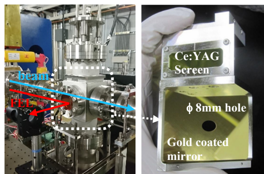
Figure 5: FEL extraction system (left) and the perforated gold-coated SUS mirror for reflecting FEL radiation (right).
