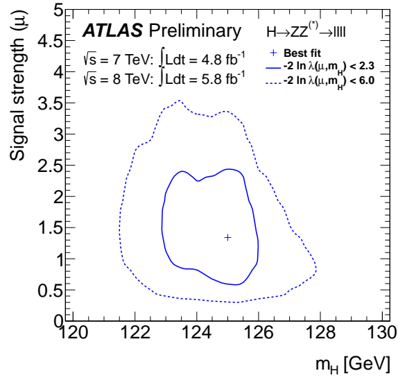
Figure 17: Best fit values for \mu and m_H , and likelihood ratio contours that, in the asymptotic limit, correspond to 68% and 95% level contours in the (\mu, m_H) plane.
