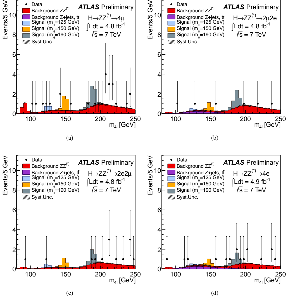
Figure 10: The distribution of the four-lepton invariant mass, m_{4\ell} , for the selected candidates for the \sqrt{s} = 7 TeV analysis for the various sub-channels (a) 4\mu , (b) 2\mu 2e , (c) 2e 2\mu , (d) 4e , compared to the background expectation for the 80–250 GeV mass range. Error bars represent 68.3% central confidence intervals. The signal expectation for several m_H hypotheses is also shown.
