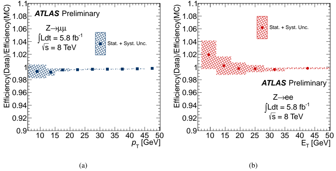
Figure 19: Ratio of the isolation and impact parameter efficiencies between data and simulation, estimated with the Tag & Probe method, using (a) Z \rightarrow \mu\mu and (b) Z \rightarrow ee events.
