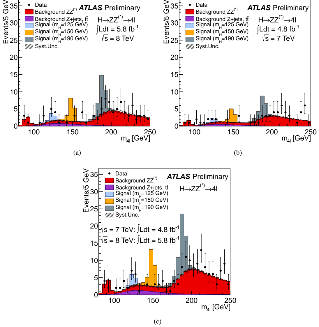
Figure 21: The distribution of the four-lepton invariant mass, m_{4\ell} , for the selected candidates compared to the background expectation for the 80–250 GeV mass range for the (a) \sqrt{s} = 8 TeV, (b) \sqrt{s} = 7 TeV and (c) combined datasets. Error bars represent 68.3% central confidence intervals. The signal expectation for several m_H hypotheses is also shown.
