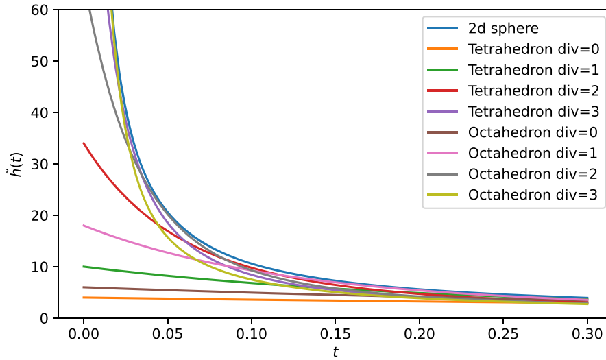
Fig. 3. Plots of the heat kernel. If the number of vertices (or faces) of the geodesic polyhedra is large, the behavior of the heat kernel becomes very close to that of the smooth two-dimensional sphere. (The “div” in the legend stands for the number of times the triangular faces of the tetrahedron or octahedron are divided into smaller triangles.)
