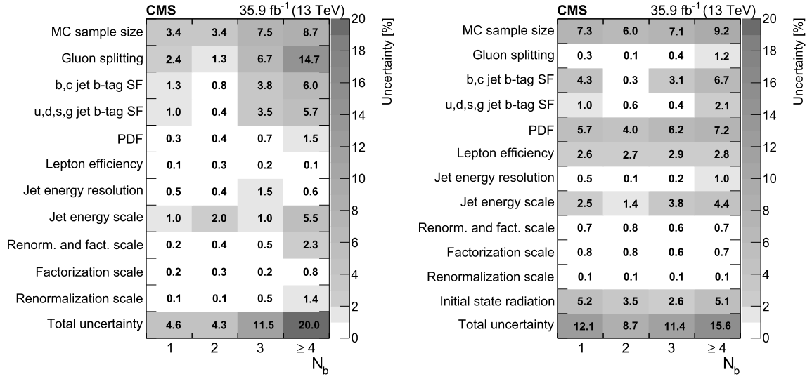
Fig. 6. Background (left) and m_{\tilde{g}} = 1600 GeV signal (right) systematic uncertainties affecting the N_b shape (in percent) in the N_{\text{jet}} \geq 8 and M_J \geq 1000 GeV bin. The bottom row shows the total uncertainty for a given N_b bin by summing in quadrature all uncertainties. These values are similar for other (N_{\text{jet}}, M_J) bins.
