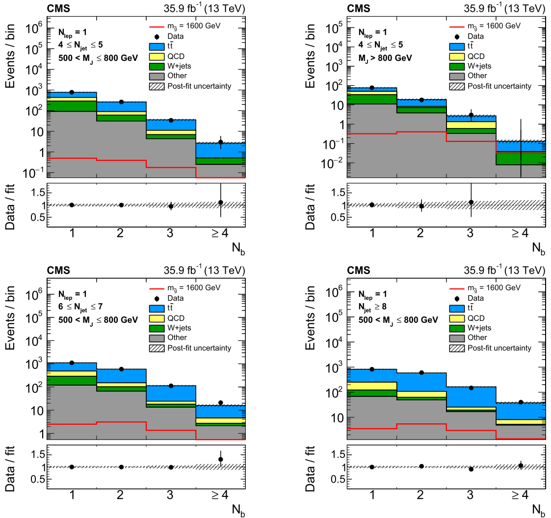
Fig. 7. Data and the background-only post-fit N_b distribution for bins with low expected signal contribution: 500 < M_J \leq 800 GeV, 4 \leq N_{\text{jet}} \leq 5 (upper-left), M_J > 800 GeV, 4 \leq N_{\text{jet}} \leq 5 (upper-right), 500 < M_J \leq 800 GeV, 6 \leq N_{\text{jet}} \leq 7 (lower-left), and 500 < M_J \leq 800 GeV, N_{\text{jet}} \geq 8 (lower-right). The expected signal distribution is also shown for a gluino mass of 1600 GeV. The ratio of data to post-fit yields is shown in the lower panel. The post-fit uncertainty is depicted as a hatched band.
