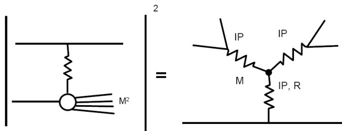
Fig. 2. Mueller's 3\mathbb{P} approximation for SD.
