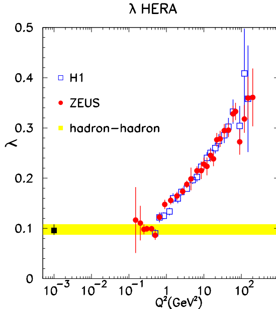
Fig. 7. Q^2 dependence of e - p DIS.
