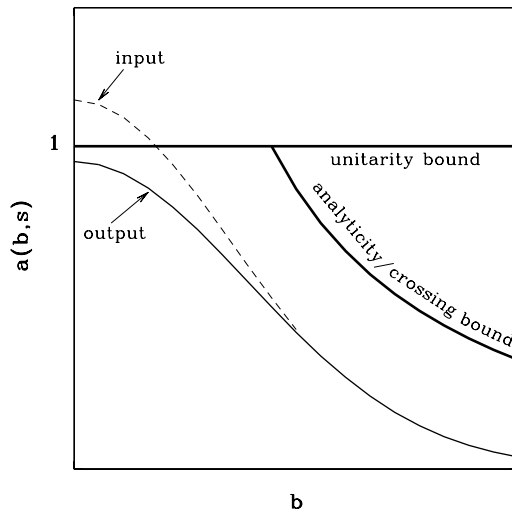
Fig. 1. The effect of eikonal screening restoring s unitarity. The bounds implied by analyticity/crossing are also shown.
