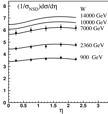
Fig. 12. GLM fit to CMS inclusive charged pseudorapidity distributions.
