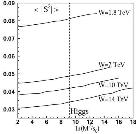
Fig. 6. GLM estimates of S^2 for exclusive central diffraction.
