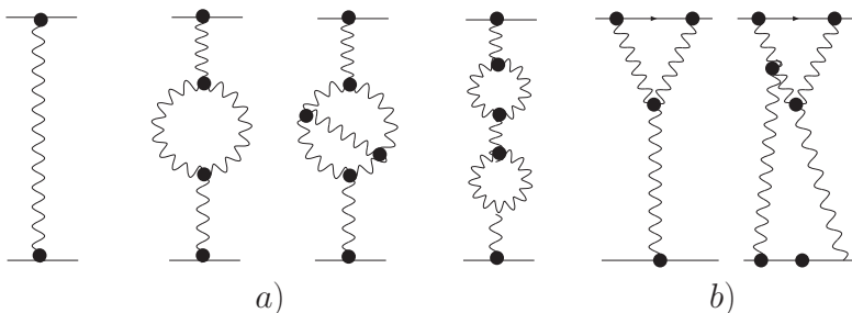
Fig. 3. The low order \mathbb{P} Green's function.
