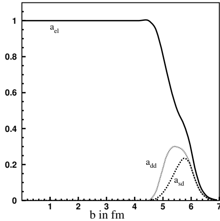
Fig. 9. GLM El, SD, and DD b -space amplitudes at the Planck scale.
