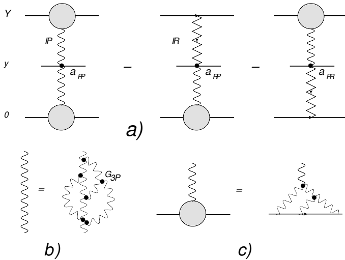
Fig. 10. (a) Mueller inclusive diagrams, (b) \mathbb{P} Green function, (c) \mathbb{P} -hadron vertex. A bold waving line = \mathbb{P} . A zigzag line = R .
