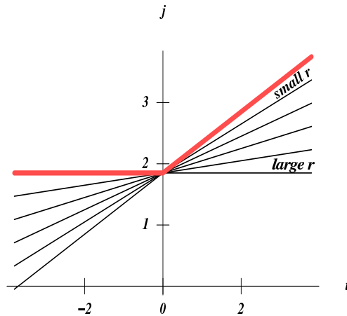
Fig. 8. The N = 4 SYM \mathbb{P} trajectory which has different slopes at positive and negative t . The figure is taken from Brower, Polchinski, Strassler and Tan.
