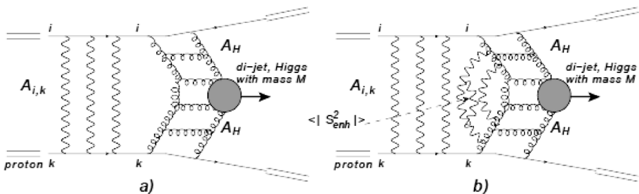
Fig. 4. An example of the screenings generating the gap survival probability for exclusive central diffractive production of the Higgs boson. (a) shows the contribution to the survival probability in the GW mechanism, while (b) illustrates the origin of the additional factor \langle |S_{\text{enh}}^2| \rangle .
