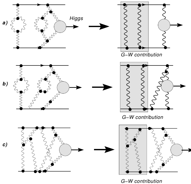
Fig. 5. GLM diagrams for exclusive central diffraction.
