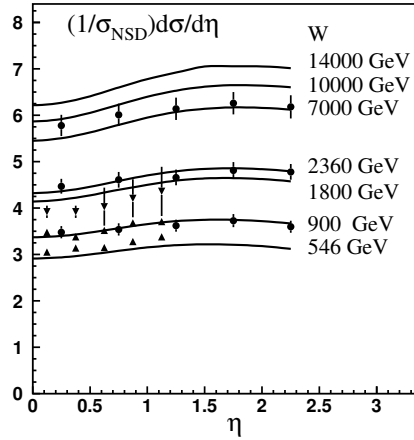
Fig. 11. GLM fit to inclusive charged pseudorapidity distributions. Data from Refs. [23, 26].
