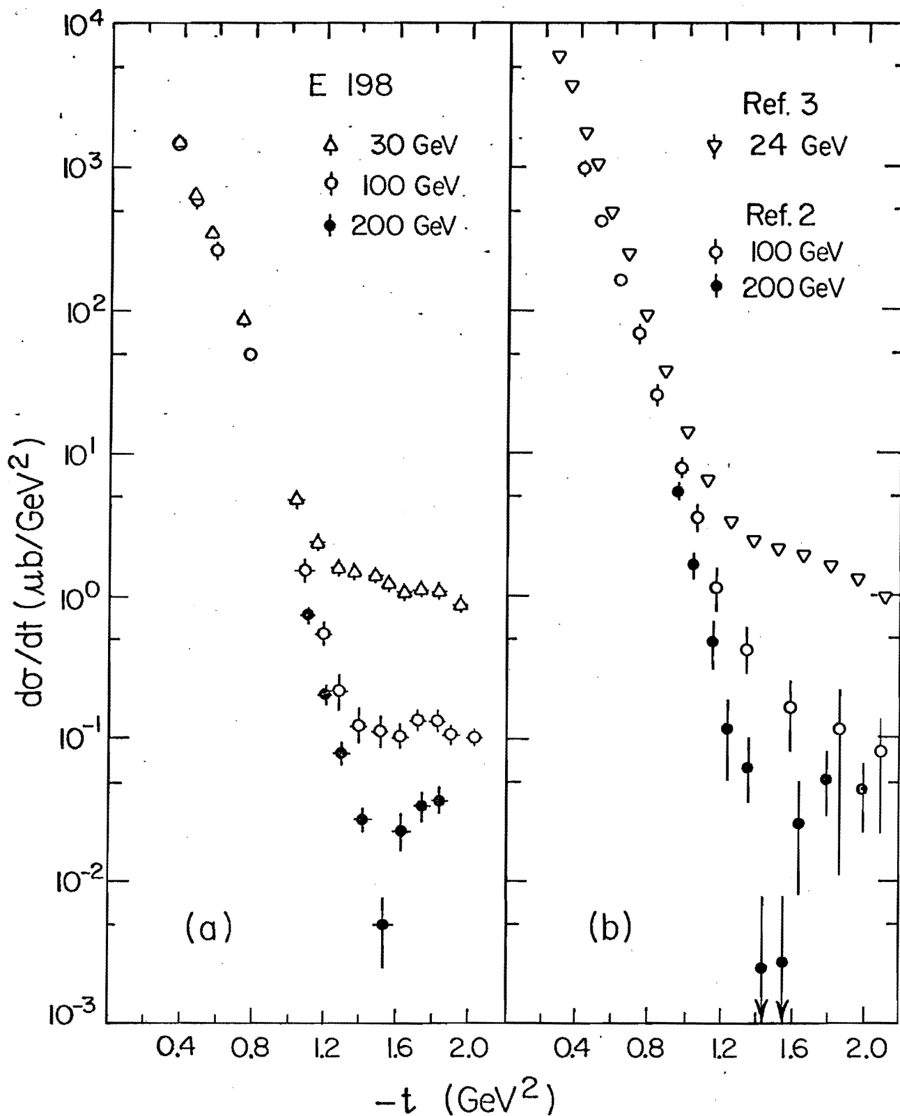
Fig. 1(a): Differential cross sections for the reaction pp \rightarrow pp as measured by E198. Full \Delta t and \Delta E bites are 0.06 \text{ GeV}^2 and 20 \text{ GeV} respectively. The cross sections were calculated from a 20% sample of the total data taken. When the full data set is analyzed we hope to have cross sections at every 20 \text{ GeV} interval between 30 and 280 \text{ GeV} with errors approaching those of the 30 \text{ GeV} data shown. Fig. 1(b): Cross sections measured in earlier experiments.
