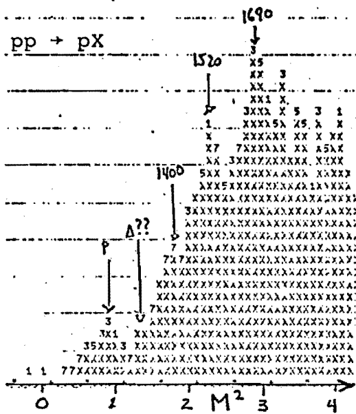
Fig. 2. Missing mass spectrum measured by E198 at -t = 1.6 \text{ GeV}^2 and E = 100 \text{ GeV} .
