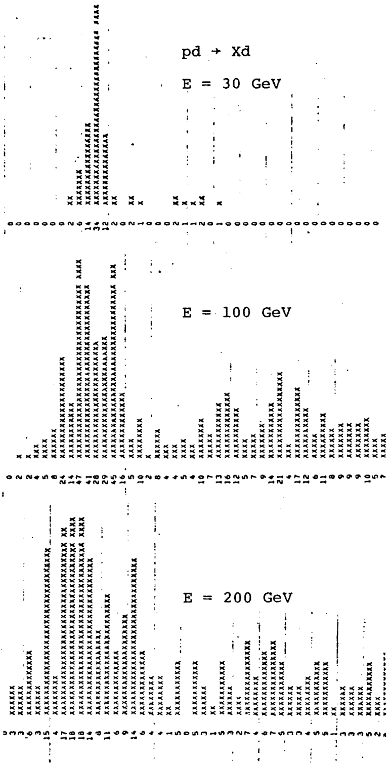
Fig. 3. Spectra of missing mass recoiling off the deuteron in pd coherent scattering at -t = 1.3 \text{ GeV}^2 and three incident energies.
