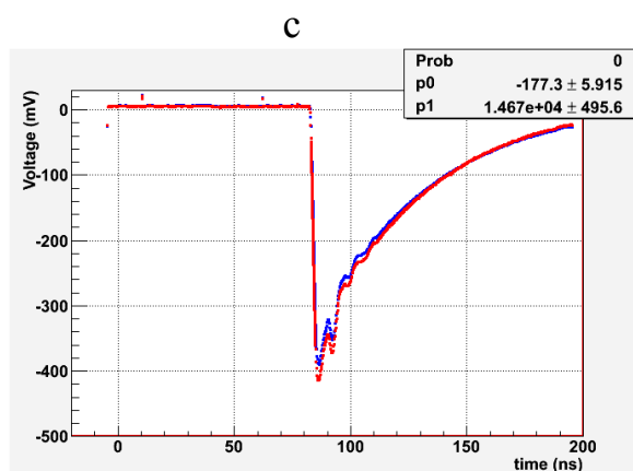
Fig. 9. Traces of 2 STMs signals (a), and 2 MPPC signals (b) taken by Tektronix oscilloscope. 10 pF clipping capacitance. LYSO crystals irradiated by radioactive source Co60, Ortec VT120C preamplifiers; c - traces of 2 MPPCs signals taken
