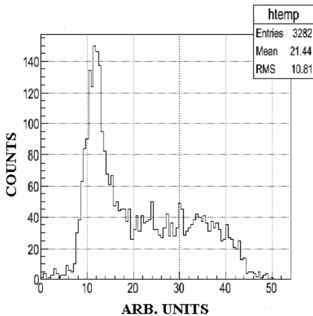
Fig. 10. Example of time (top) and pulse height (bottom) distribution. The conditions: Hamamatsu MPPC, 3 \times 3 \text{ mm}^2 ; LYSO crystal, 2 \times 2 \times 7 \text{ mm}^3 ; VT120C amplifier, Co60 radioactive source. 155 ps (sigma) time resolution.
