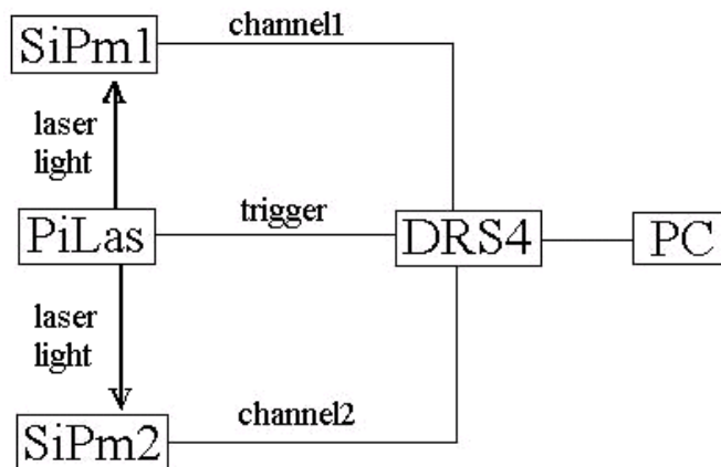
Fig. 4. The schematic diagram of the readout with the PiLas laser. SiPm1, 2 – silicon photomultipliers, PiLas – picoseconds laser, DRS4 – waveform digitizer, PC – personal computer.
