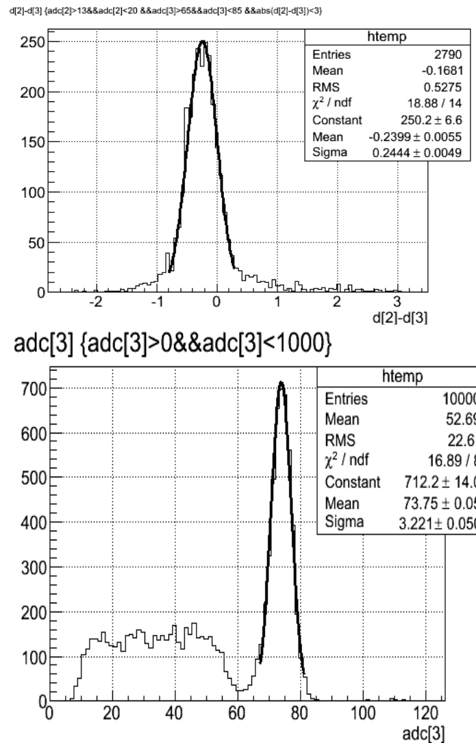
Fig. 11. Example of time (top) and pulse height (bottom) distribution. The conditions: Hamamatsu MPPC, 3 \times 3 \text{ mm}^2 ; LYSO crystal, 3 \times 3 \times 15 \text{ mm}^3 ; VT120C amplifier, Na22 radioactive source. 244 ps (sigma) time resolution, 10% (FWHM) photo peak resolution.
