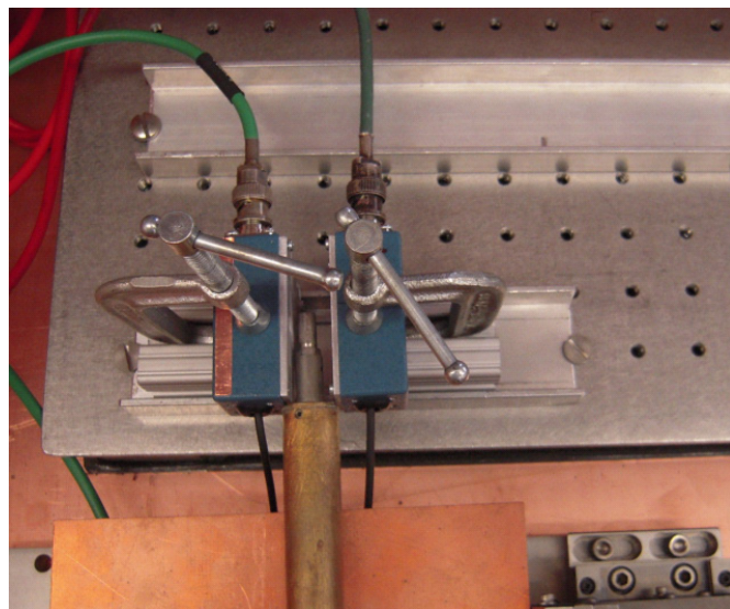
Fig. 7. External view of the TOF-PET setup.
