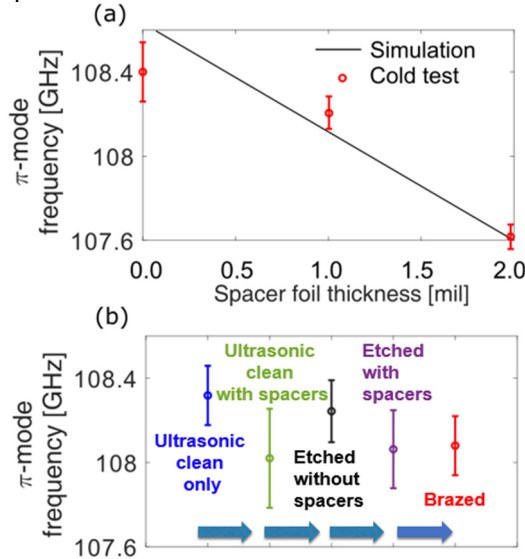
Figure 2: (a) Simulation versus cold test results of the \pi -mode resonance frequency varying as a function of the spacer foil thickness. (b) Measured frequency of the \pi -mode throughout the various braze processes.
