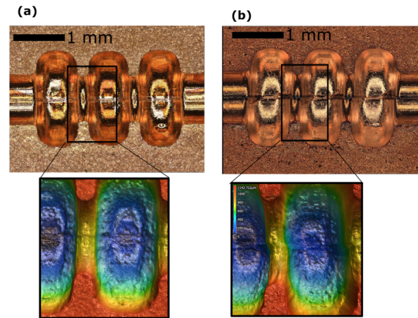
Figure 3: Photo of two sectioned samples of W-band accelerator cavities after brazing (top), and zoomed in images of the surface topology of the cavity (bottom).
