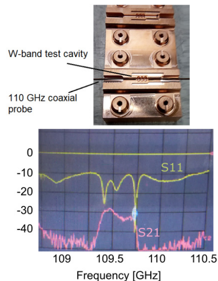
Figure 1: Photo of one of the W-band blocks for braze test (top), and the S parameters measured using mm-wave vector network analyzer with coaxial probes (bottom).
