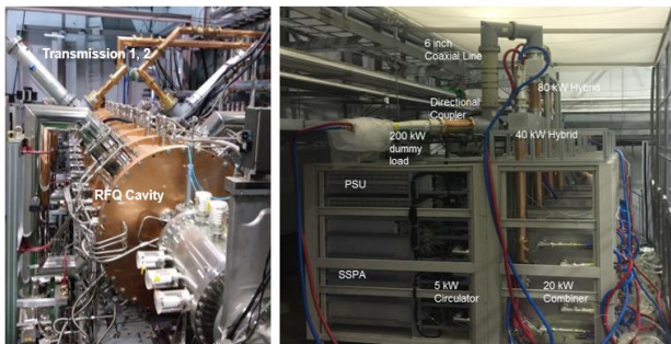
Figure 7: RFQ cavity, transmission lines and SSPAs for RFQ RF conditioning.
