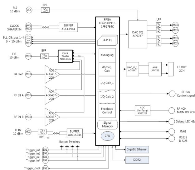
Figure 1: Block diagram of 81.25 MHz LLRF module.
