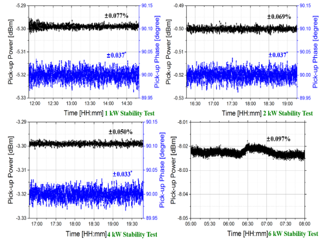
Figure 5: RF amplitude and phase stability.
