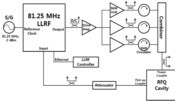
Figure 3: Block diagram of test bench for stability test
