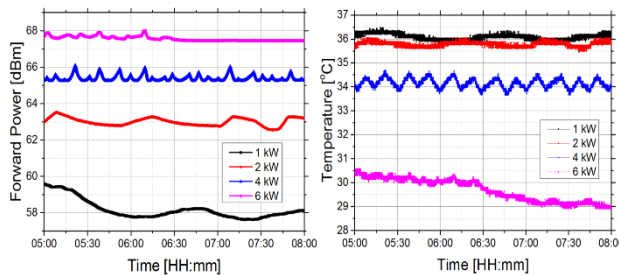
Figure 4: Forward power and temperature of RCCS during the stability test.
