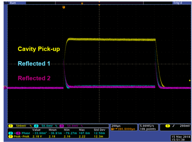
Figure 8: Measured RFQ field and reflected power in pulsed mode.
