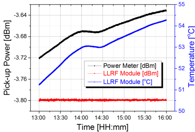
Figure 6: Correlation between pick-up power and temperature of LLRF module.
