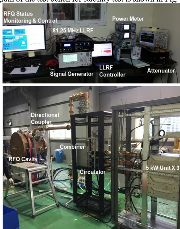
Figure 2: Test setup with 81.25 MHz LLRF, 15 kW SSPA and RFQ cavity.
