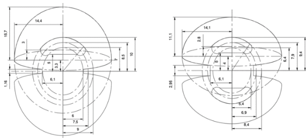
Figure 3: Geometric structure of cross section, main part(left) and transition part(right).
