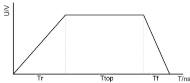
Figure 1: Simplified input pulse profile.
