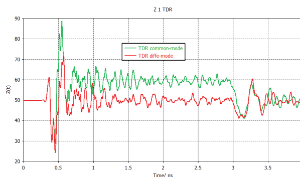
Figure 6: TDR in simulation.
