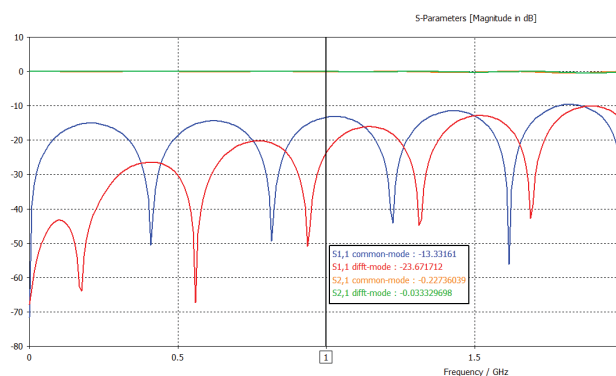
Figure 5: S-parameters in simulation.
