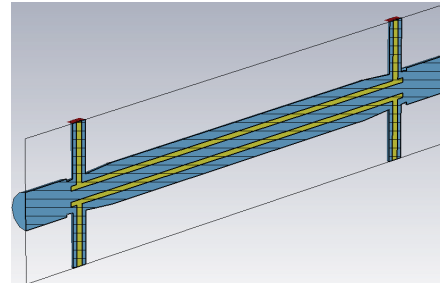
Figure 2: Overall structure of kicker.
