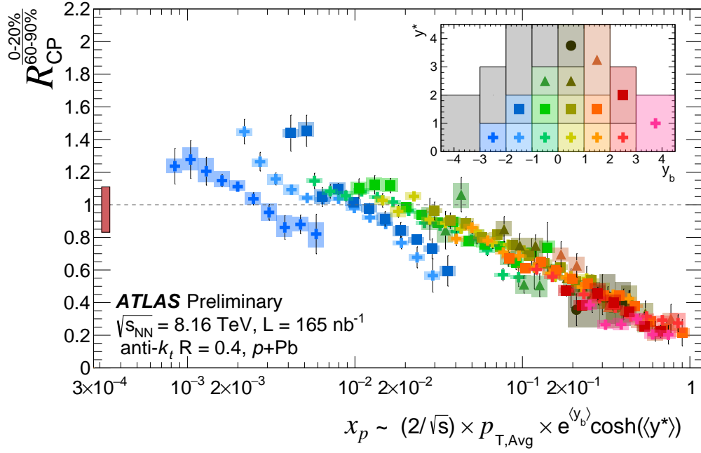
Figure 14: R_{\text{CP}} plotted as a function of approximated x_p , constructed using \langle y_b \rangle and \langle y^* \rangle . An inlay legend is included, showing the (y_b, y^*) bins, and their corresponding markers and colors. Note that positive y_b corresponds to the proton-going direction. Colored rectangles represent the total systematic uncertainty, while the vertical black error bars represent the statistical uncertainty. The solid red rectangle on the left-side of the panel represents the uncertainty on the T_{\text{AB}} . Four (y_b, y^*) bins, denoted in the legend by a grey color and no marker, were dropped from the analysis as the presence of jets in these intervals, which are nearby to the forward calorimeter, may bias the centrality determination.
