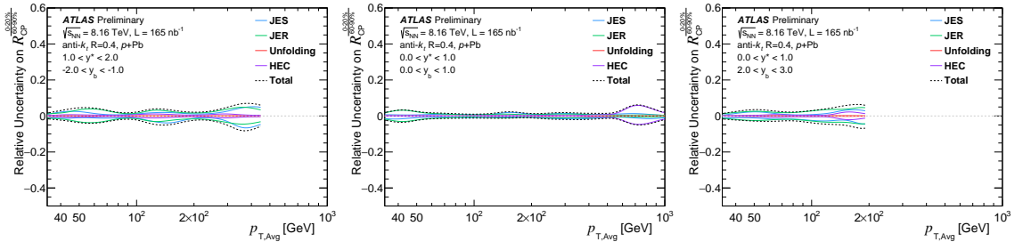
Figure 8: The systematic uncertainties on the R_{CP} measurement as a function of p_{T,Avg} in three representative bins of y_b and y^* for \sqrt{s_{NN}} = 8.16 TeV p+Pb collisions. Each panel shows the total systematic uncertainty (black dashed line), as well as the contributions from each source, namely the JES, JER, unfolding, and HEC sector exclusion. The T_{AB} uncertainty (not displayed) has a value of +10% and –16% in all bins.
