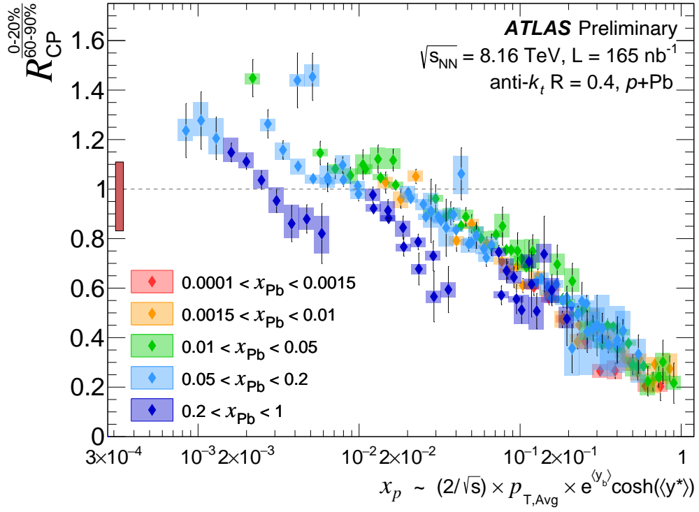
Figure 16: R_{\text{CP}} plotted as a function of approximated x_p , in different ranges of approximated x_{\text{Pb}} , both constructed using \langle y_b \rangle and \langle y^* \rangle . Note that positive y_b corresponds to the proton-going direction. Colored rectangles represent the total systematic uncertainty, while the vertical black error bars represent the statistical uncertainty. The solid red rectangle on the left side of the panel represents the uncertainty on the T_{\text{AB}} .
