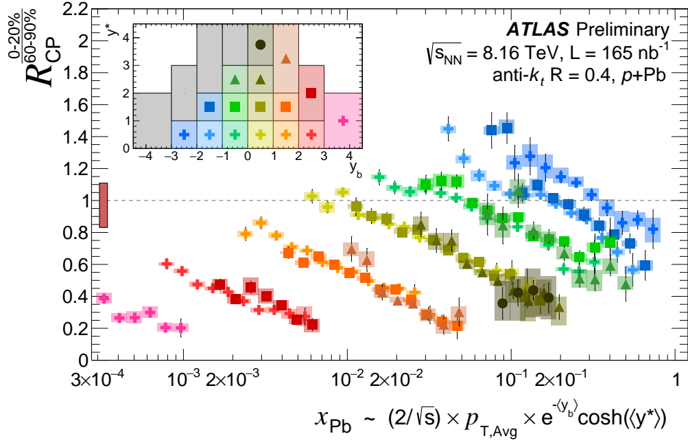
Figure 15: R_{\text{CP}} plotted as a function of approximated x_{\text{Pb}} , constructed using \langle y_b \rangle and \langle y^* \rangle . An inlay legend is included, showing the (y_b, y^*) bins, and their corresponding markers and colors. Note that positive y_b corresponds to the proton-going direction. Colored rectangles represent the total systematic uncertainty, while the vertical black error bars represent the statistical uncertainty. The solid red rectangle on the left-side of the panel represents the uncertainty on the T_{\text{AB}} . Four (y_b, y^*) bins, denoted in the legend by a grey color and no marker, were dropped from the analysis as the presence of jets in these intervals, which are nearby to the forward calorimeter, may bias the centrality determination.
