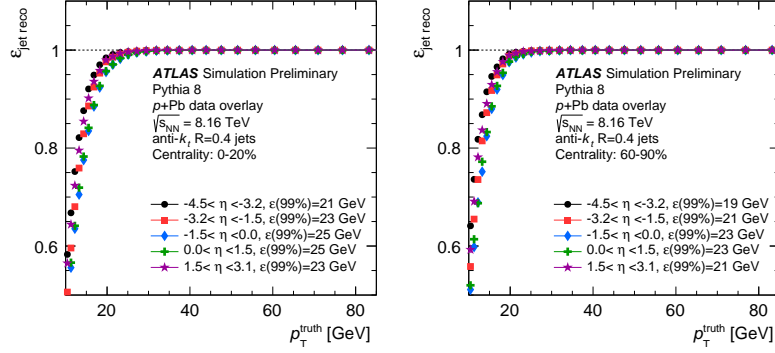
Figure 4: Jet reconstruction efficiency in p+\text{Pb} data-taking configuration, evaluated in different \eta regions of the ATLAS detector for central (0–20%, left) and peripheral (60–90%, right) collisions. All jets with p_T^{\text{reco}} > 5 GeV were considered in these studies. Corresponding 99% efficiency p_T^{\text{truth}} thresholds are also reported for each \eta region and centrality interval.
