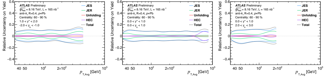
Figure 7: The systematic uncertainties on the 60–90% per-event dijet yield measurement as a function of p_{T,Avg} in three representative bins of y_b and y^* for \sqrt{s_{NN}} = 8.16 TeV p+Pb collisions. Each panel shows the total systematic uncertainty (black dashed line), as well as the contributions from each source, namely the JES, JER, unfolding and disabled HEC sector.
