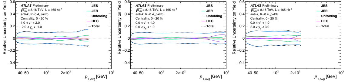
Figure 6: The systematic uncertainties on the 0–20% per-event dijet yield measurement as a function of p_{T,Avg} in three representative bins of y_b and y^* for \sqrt{s_{NN}} = 8.16 TeV p+Pb collisions. Each panel shows the total systematic uncertainty (black dashed line), as well as the contributions from each source, namely the JES, JER, unfolding and disabled HEC sector.
