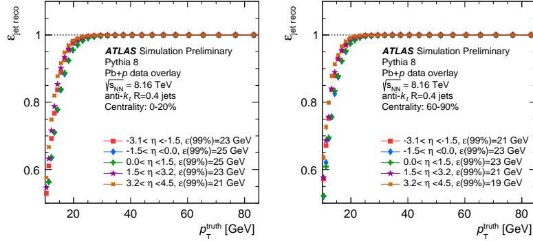
Figure 5: Jet reconstruction efficiency in \text{Pb}+p data-taking configuration, evaluated in different \eta regions of the ATLAS detector for central (0–20%, left) and peripheral (60–90%, right) collisions. All jets with p_T^{\text{reco}} > 5 GeV were considered in these studies. Corresponding 99% efficiency p_T^{\text{truth}} thresholds are also reported for each \eta region and centrality interval.
