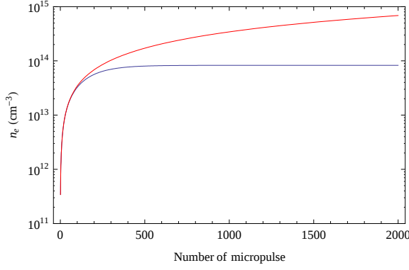
FIG. 7: Examples of electron density evolution over many micropulses without (red) and with (blue) recombination. Here, we pick the parameters to \beta_r \sim 10^{-8} \text{cm}^3 \text{s}^{-1} , r_b \sim 1 \text{ cm} , p = 500 \text{ psi} .
