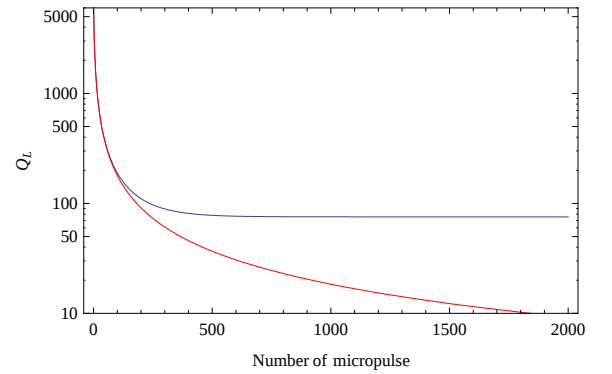
FIG. 8: Decrease in the loaded Q , Q_L , over many micropulses without (red) and with (blue) considering recombination process. Initially, we assume Q_L = 6000 .
