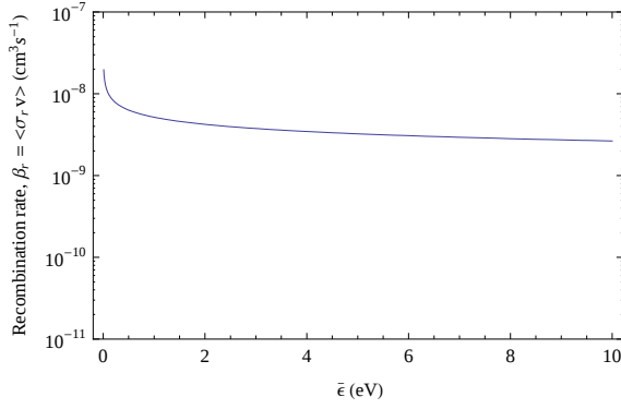
FIG. 6: Dissociative recombination rate coefficient as a function of average electron energy [19, 20].
