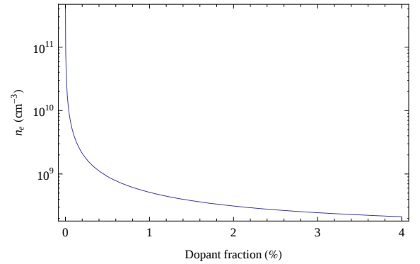
FIG. 10: Equilibrium electron density as a function of dopant fraction for k_a \approx 2 \times 10^{-9} \text{ cm}^3 \text{ s}^{-1} and \delta_e \approx 10 \times (2m_e/m_{H_2}) .
