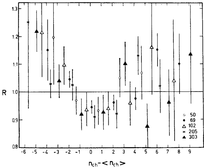
Fig. 13. Ratio R (see Fig. 12) as a function of n - \langle n \rangle . Experimental data are from the range 50 GeV/c < p_{LAB} < 303 GeV/c
