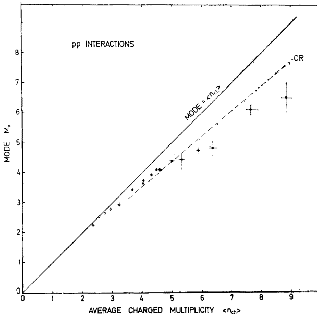
Fig. 15. Mode M_0 as a function of \langle n \rangle for pp collisions. The dashed line (CR) has been calculated from the Czyżewski-Rybecki formula with d = 1.7 . The decrease in d decreases the slope of the dashed line
