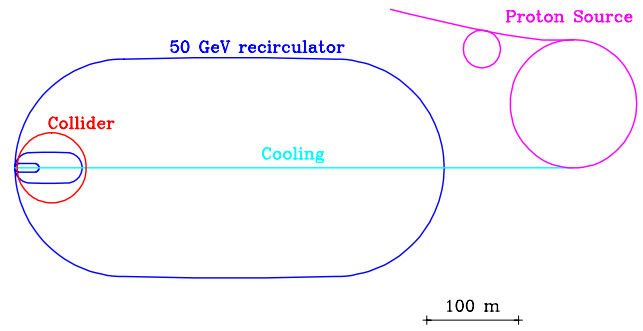
Figure 1: Plan of a 100 GeV Muon Collider.
