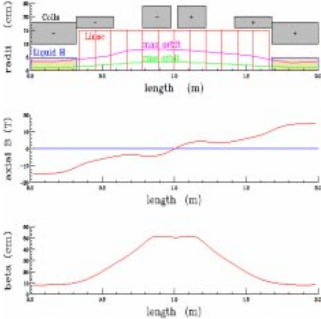
Figure 3: a) Cross section of one cell (2 m) of an alternating solenoid cooling system; b) axial magnetic field vs. z ; c) beta function vs. z .
