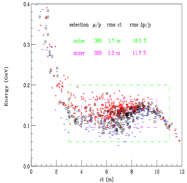
Figure 2: Kinetic energy vs. ct of muons at end of phase rotation channel. The symbols +, o and - denote muons with polarization P > \frac{1}{3} , -\frac{1}{3} < P < \frac{1}{3} and P < -\frac{1}{3} , respectively.
