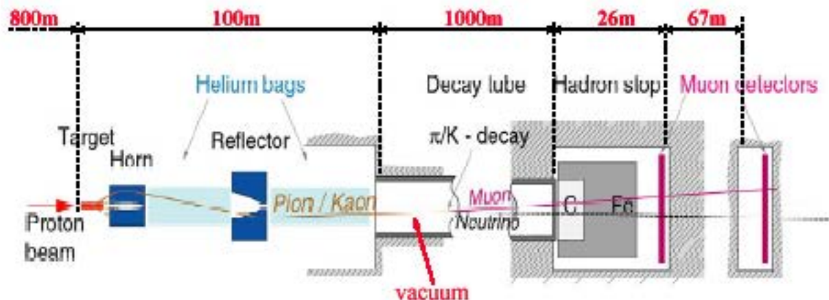
Figure 1: CNGS layout.
