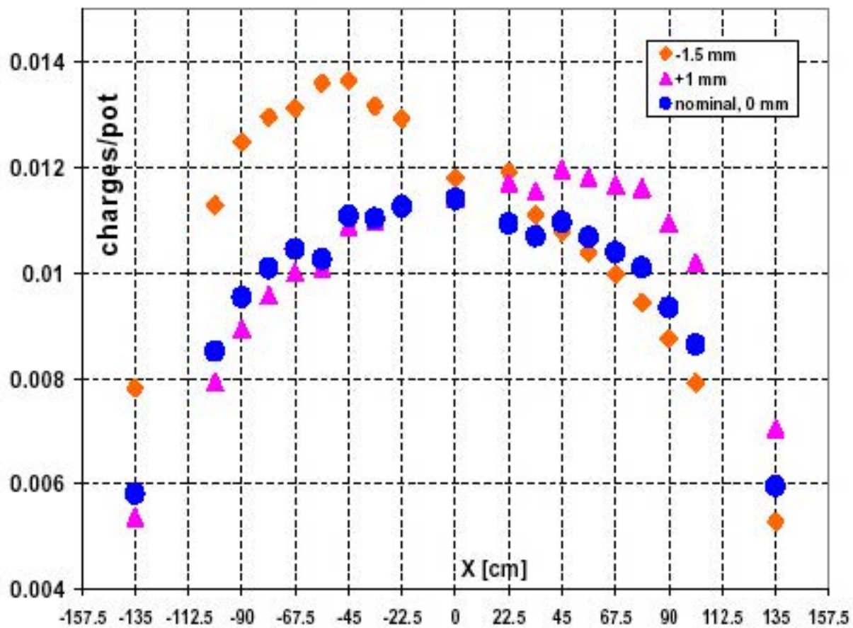
Figure 2: Vertical muon profile in the second muon detector chamber for different beam versus target alignments (0mm, +1mm, -1.5mm). Each point corresponds to a detector and shows the measured induced charges per proton on target ( \sim 2700 charges/muon are produced in a detector). The statistical accuracy is limited (as indicated by the fluctuations of the data points) because the dynamic range of the readout electronics is adjusted to the nominal CNGS intensity ( 2.4 \cdot 10^{13} p.o.t./extraction). The measurements were performed with \sim 2 \cdot 10^{12} p.o.t./extraction.
