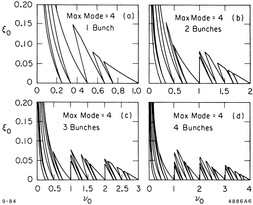
FIGURE 6 Same as Fig. 4 but taking into account resonances up to order 4.
