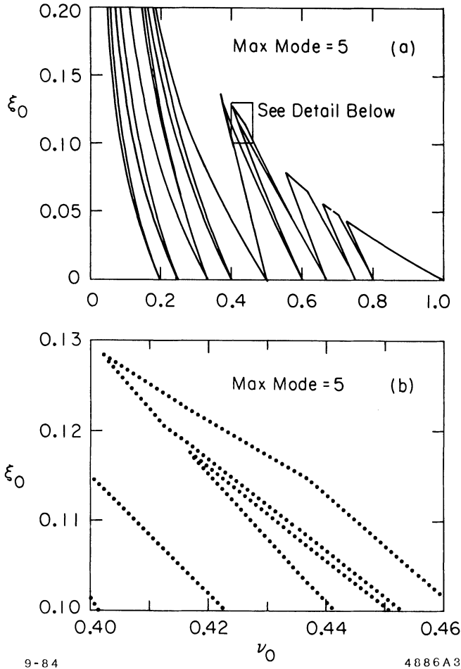
FIGURE 3 (a) Stability diagrams for one bunch per beam including resonances through order 5. (b) Blow up of a portion of (a) showing some interference behavior between adjacent resonances.
