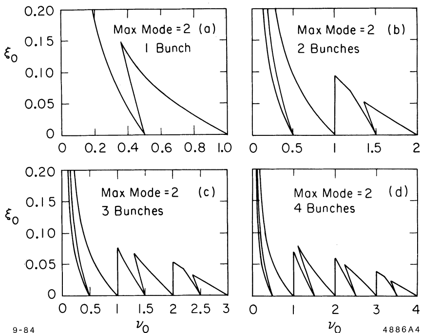
FIGURE 4 Stability diagrams for the cases of 1, 2, 3 and 4 bunches per beam, taking into account dipole and quadrupole resonances.
