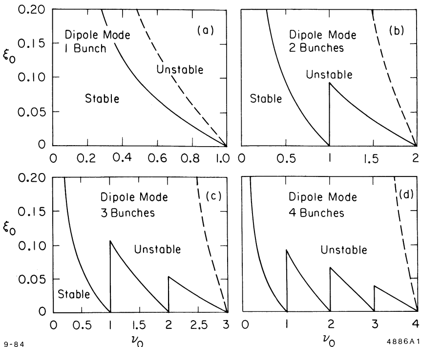
FIGURE 1 Stability diagrams in (\nu_0, \xi_0) space, where \nu_0 is the unperturbed tune for the storage ring and \xi_0 is the beam-beam strength parameter, for the cases with 1, 2, 3 and 4 bunches per beam. The beam bunches are regarded as rigid allowing only dipole coherent motions.
