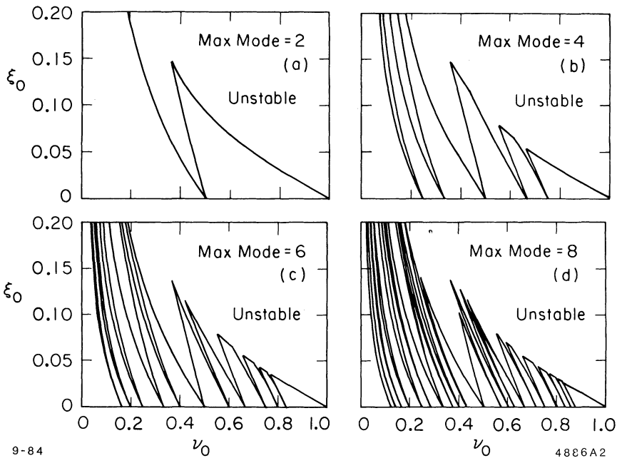
FIGURE 2 Stability diagrams for the case of one bunch per beam. In each of the four plots resonances up to order 2, 4, 6 and 8 are included, respectively.
