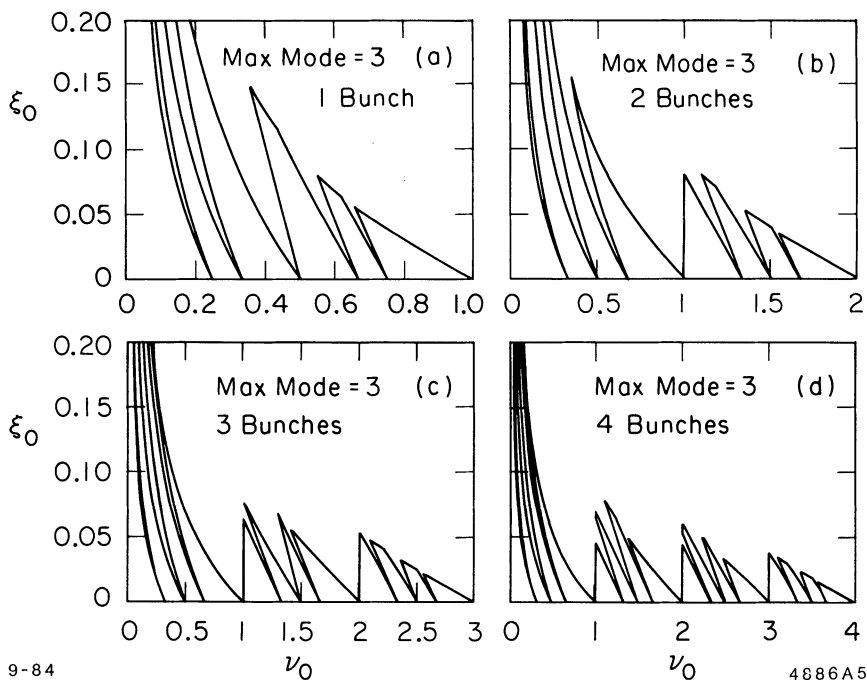
FIGURE 5 Same as Fig. 4 but taking into account resonances up to order 3.
