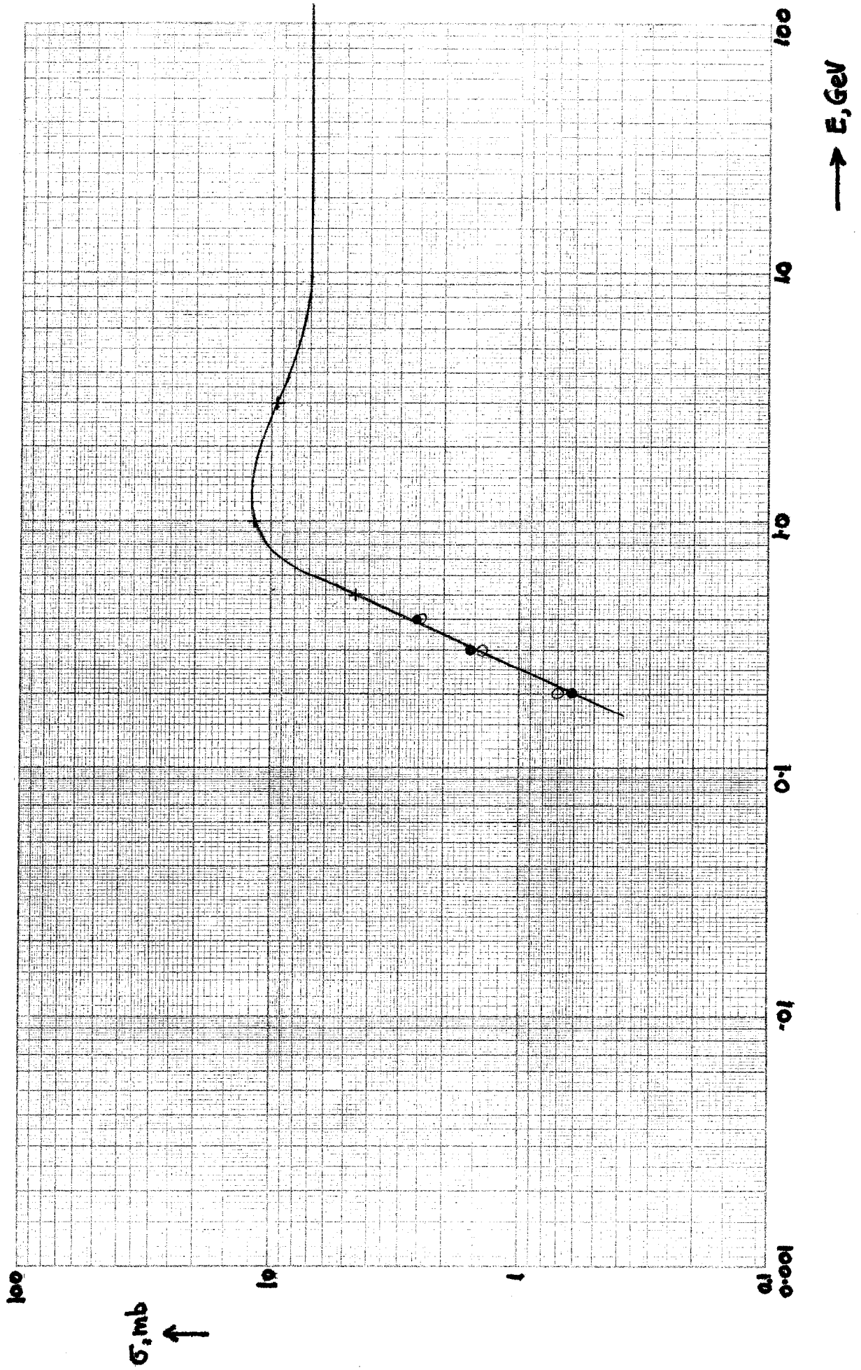
Fig. 5. \text{Na}^{22} excitation function for \text{Ca(K)} .
