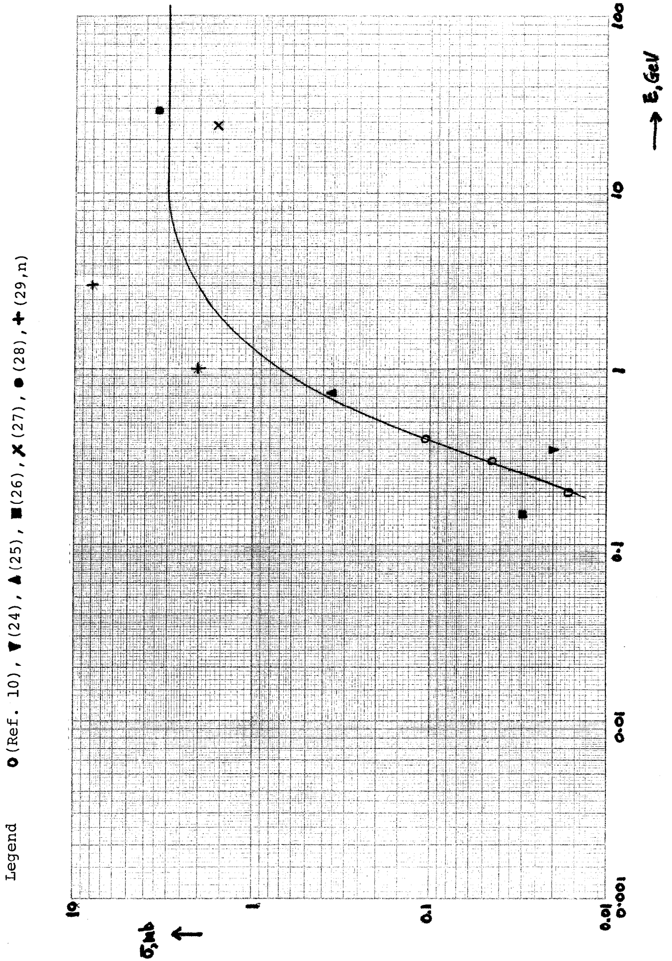
Fig. 6. \text{Na}^{22} excitation function from Fe.
