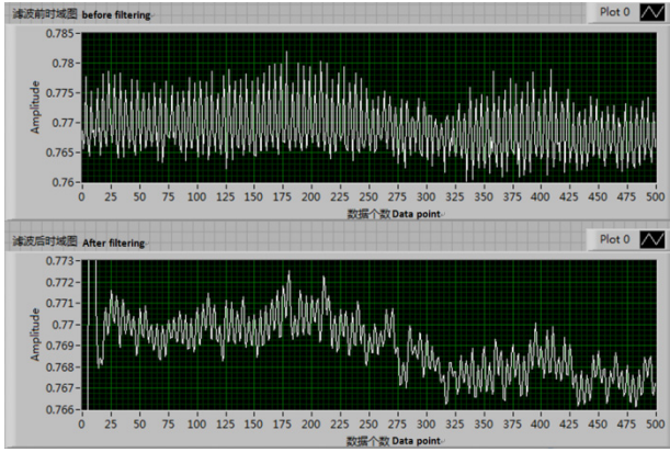
Figure 6: 500 Data samples in one test position before filtering and after filtering.
