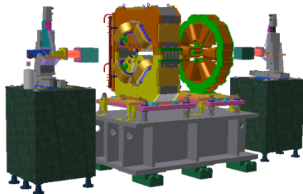
Figure 4: Vibrating wire alignment system model.
