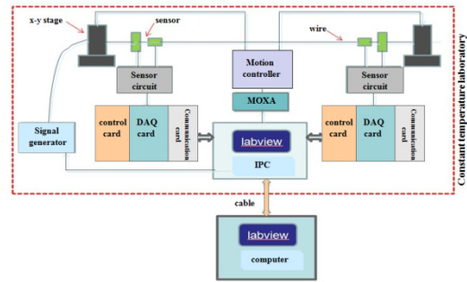
Figure 5: Scheme of motion control and data acquisition system.
