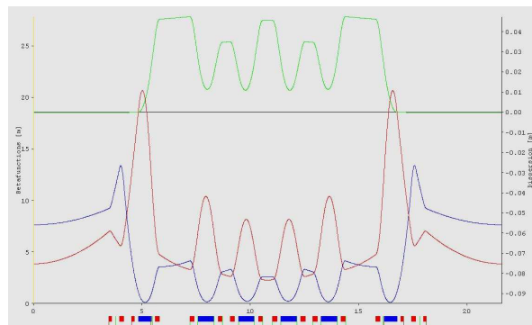
Figure 1: Elettra2.0 lattice 1.
