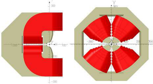
Figure 6: Dipole and quadrupole profiles.
