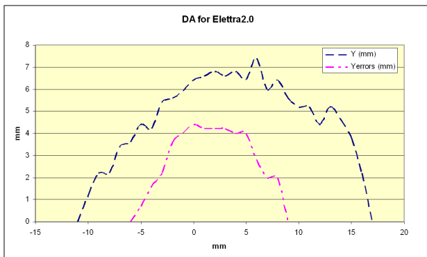
Figure 3: DA of the lattice with and without errors.
