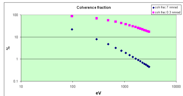
Figure 5: Coherence fraction for Elettra and Elettra2.0.
