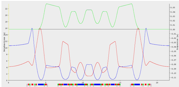
Figure 2: Elettra2.0 lattice 2 with 2 permanent magnets.
