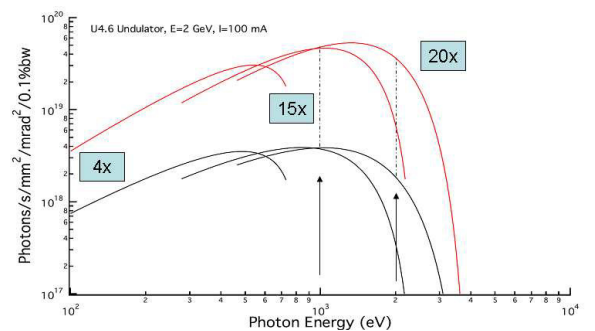
Figure 4: Brilliance increase between the actual machine and Elettra2.0.
