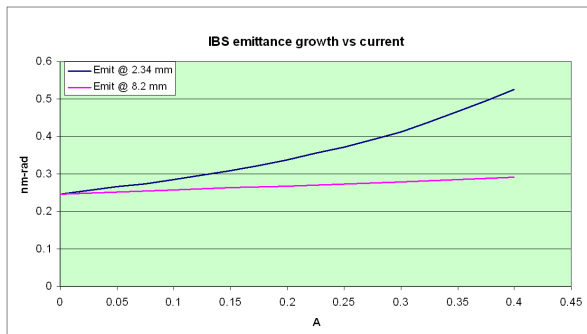
Figure 8: Emittance growth due to intra beam scattering for the natural and for a lengthened bunch due to the third harmonic cavity already in function at Elettra.
