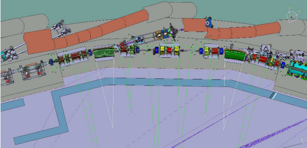
Figure 7: Elements of one sector Elettra2.0 (yellow lines) superimposed on an actual sector. Observe the short permanent magnet exactly before the actual dipole.
