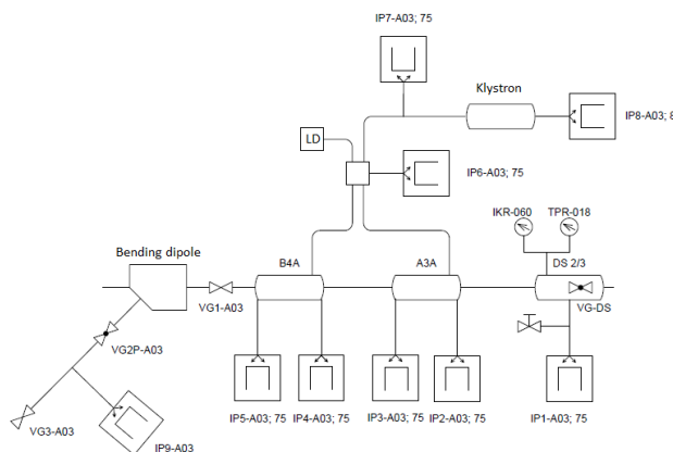
Figure 2: Vacuum system layout of one linac station.
