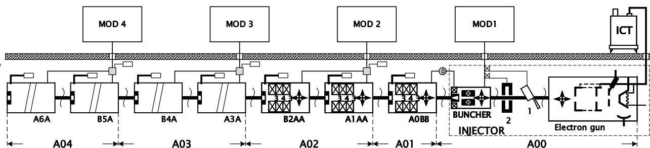
Figure 1: Linac-200 accelerator layout.
