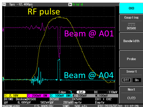
Figure 3: Beam current signal from the current transformer after A01 (magenta) and A04 (cyan) stations, and RF pulse (yellow).
