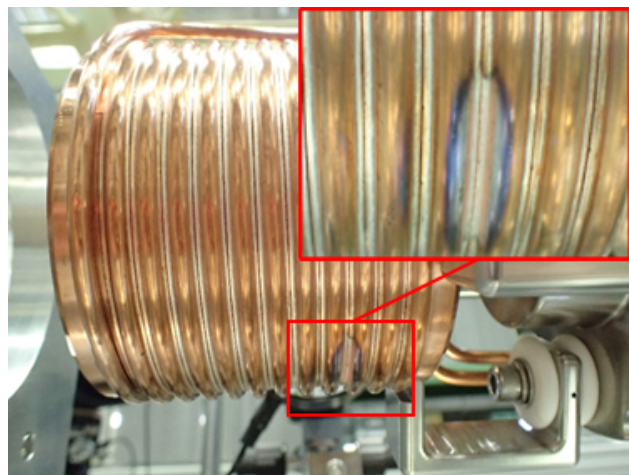
Figure 1: Typical discharge mark.
