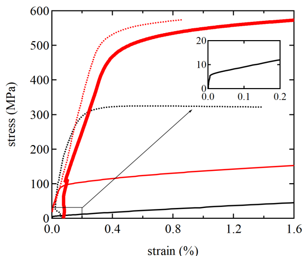
Figure 4: A strain-stress graph of NC50 (red) and C1020 (black). Dashed line shows the results before heat cycle and solid lines show the results after heat cycle. Thick red solid line shows the result of NC50 after heat cycle and aging. Inset shows expansion around origin.
