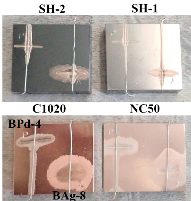
Figure 3: Results of brazing test.
