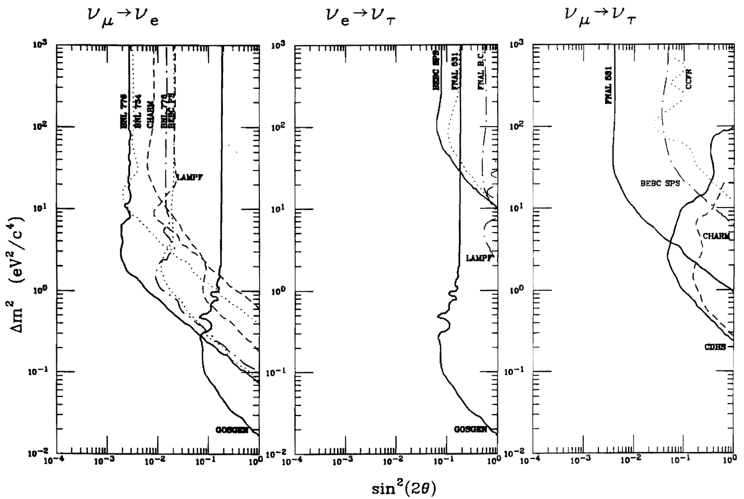
Fig. II.1: Current neutrino oscillation limits for a) \nu_\mu \rightarrow \nu_e , b) \nu_e \rightarrow \nu_\tau , and c) \nu_\mu \rightarrow \nu_\tau .
