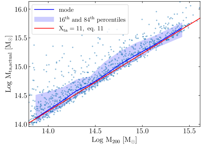
Fig. 4. Correlation between turnaround mass M_{ta,actual} and collapsed mass M_{200} for the MDPL2 cluster sample at z = 0 . The red solid line depicts the theoretical scaling relation of Eq. (11). The blue solid line represents the mode value of the blue points in bins of M_{200} . The blue shaded region corresponds to the 16th and 84th percentiles.
