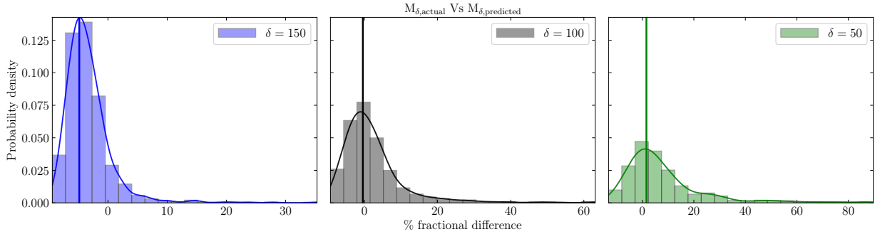
Fig. 6. Performance of our scaling relation for masses corresponding to different overdensity values \delta (equivalent to X in Eq. (11)) in the MDPL2 sample. The solid curves and vertical lines are the same as in Fig. 5. As \delta decreases (left to right), the most probable offset decreases, while high-error tails become more pronounced. Both behaviors can be traced to the performance of the analytic profile (see text for discussion).
