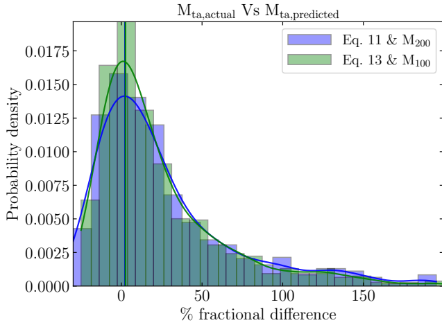
Fig. 8. Comparison between the scaling relations delineated in Eqs. (13) and (11). The blue histogram depicted herein corresponds to that of the left panel in Fig. 5. Superimposed on this histogram is the fractional difference between the actual value of M_{ta} ( X = 11 ) and its predicted counterpart assuming a prior knowledge of M_{100} (that is, if we set Y = 100 ).
